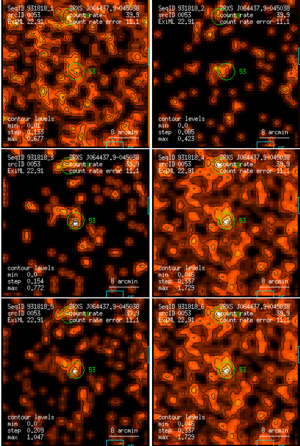
Figure 53: RASS 931818: detection 0053: band rate images, Gaussian filter: (1) PSPC channels 11 – 41, (2) 52 – 90, (3) 91 – 201, (4) 11 – 235, (5) 52 – 201, (6) 11 – 201. Broad band rates in counts/ks. Band rate contour levels in counts/ks/arcmin 2 .
