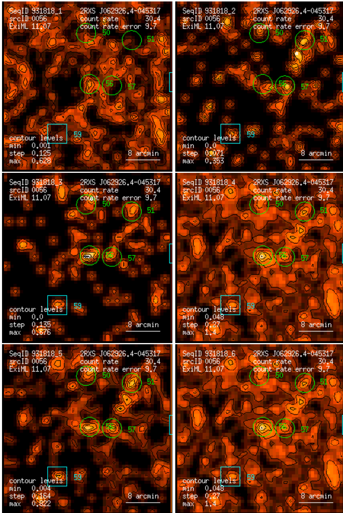
Figure 56: RASS 931818: detection 0056: band rate images, Gaussian filter: (1) PSPC channels 11 – 41, (2) 52 – 90, (3) 91 – 201, (4) 11 – 235, (5) 52 – 201, (6) 11 – 201. Broad band rates in counts/ks. Band rate contour levels in counts/ks/arcmin 2 .
