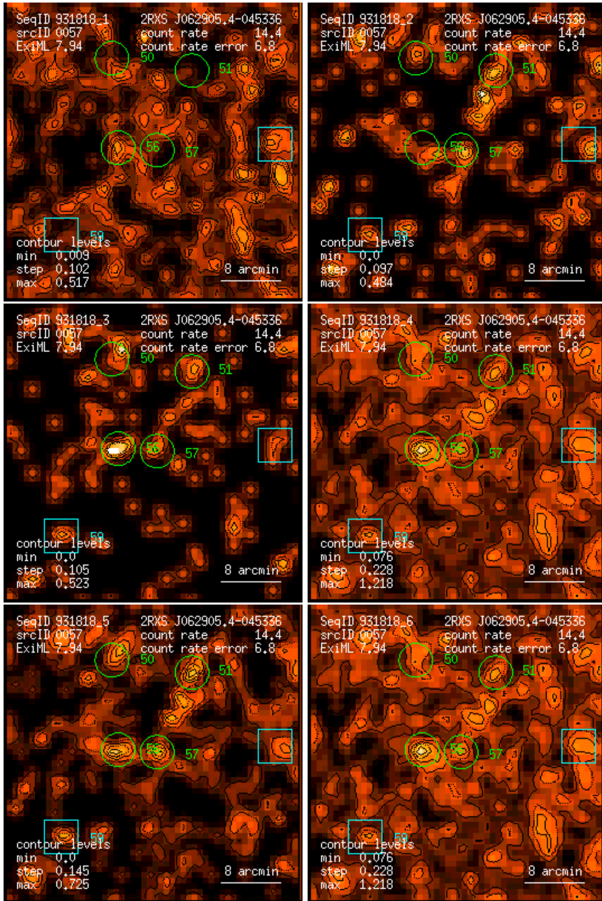
Figure 57: RASS 931818: detection 0057: band rate images, Gaussian filter: (1) PSPC channels 11 – 41, (2) 52 – 90, (3) 91 – 201, (4) 11 – 235, (5) 52 – 201, (6) 11 – 201. Broad band rates in counts/ks. Band rate contour levels in counts/ks/arcmin 2 .
