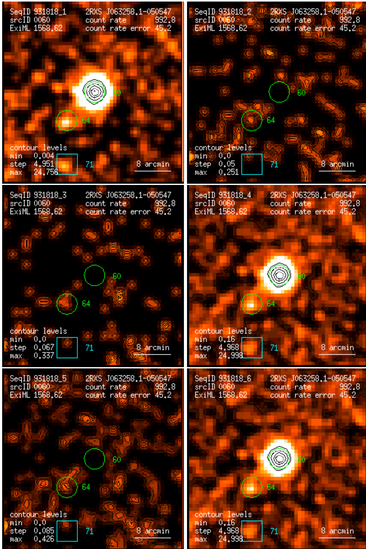
Figure 60: RASS 931818: detection 0060: band rate images, Gaussian filter: (1) PSPC channels 11 – 41, (2) 52 – 90, (3) 91 – 201, (4) 11 – 235, (5) 52 – 201, (6) 11 – 201. Broad band rates in counts/ks. Band rate contour levels in counts/ks/arcmin 2 .
