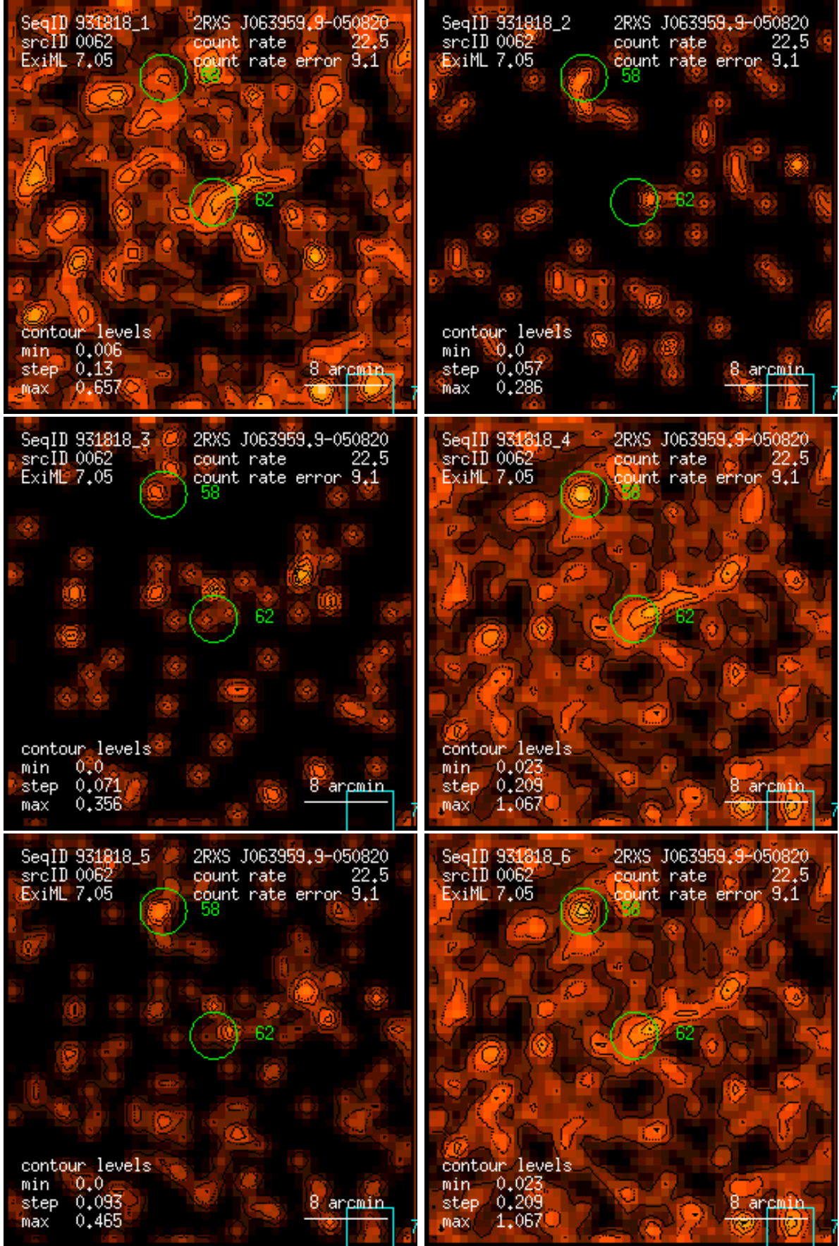
Figure 62: RASS 931818: detection 0062: band rate images, Gaussian filter: (1) PSPC channels 11 – 41, (2) 52 – 90, (3) 91 – 201, (4) 11 – 235, (5) 52 – 201, (6) 11 – 201. Broad band rates in counts/ks. Band rate contour levels in counts/ks/arcmin 2 .
