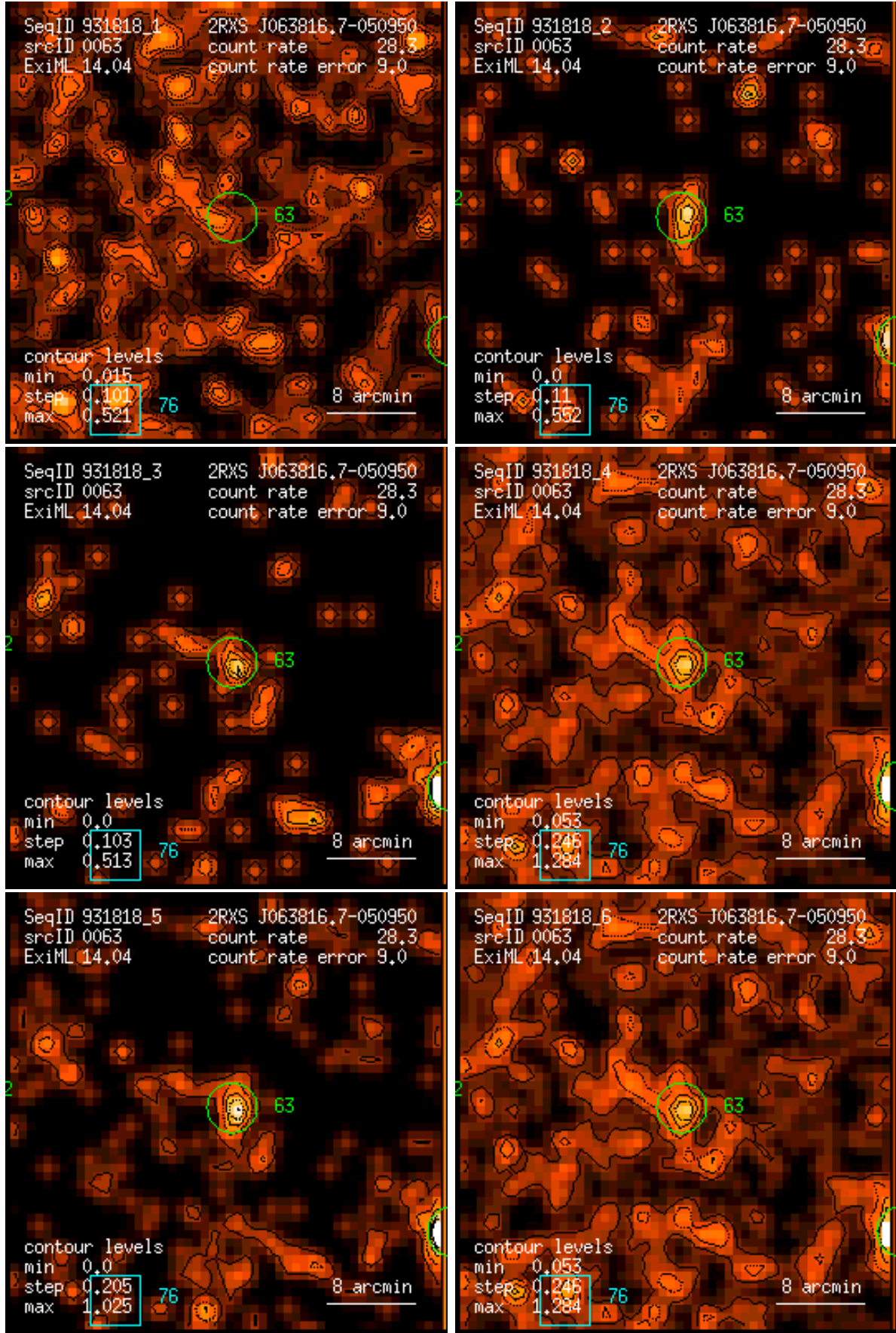
Figure 63: RASS 931818: detection 0063: band rate images, Gaussian filter: (1) PSPC channels 11 – 41, (2) 52 – 90, (3) 91 – 201, (4) 11 – 235, (5) 52 – 201, (6) 11 – 201. Broad band rates in counts/ks. Band rate contour levels in counts/ks/arcmin 2 .
