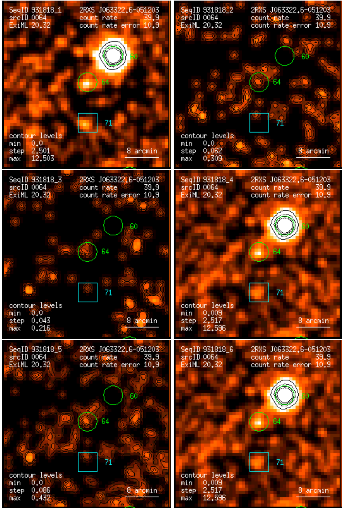
Figure 64: RASS 931818: detection 0064: band rate images, Gaussian filter: (1) PSPC channels 11 – 41, (2) 52 – 90, (3) 91 – 201, (4) 11 – 235, (5) 52 – 201, (6) 11 – 201. Broad band rates in counts/ks. Band rate contour levels in counts/ks/arcmin 2 .
