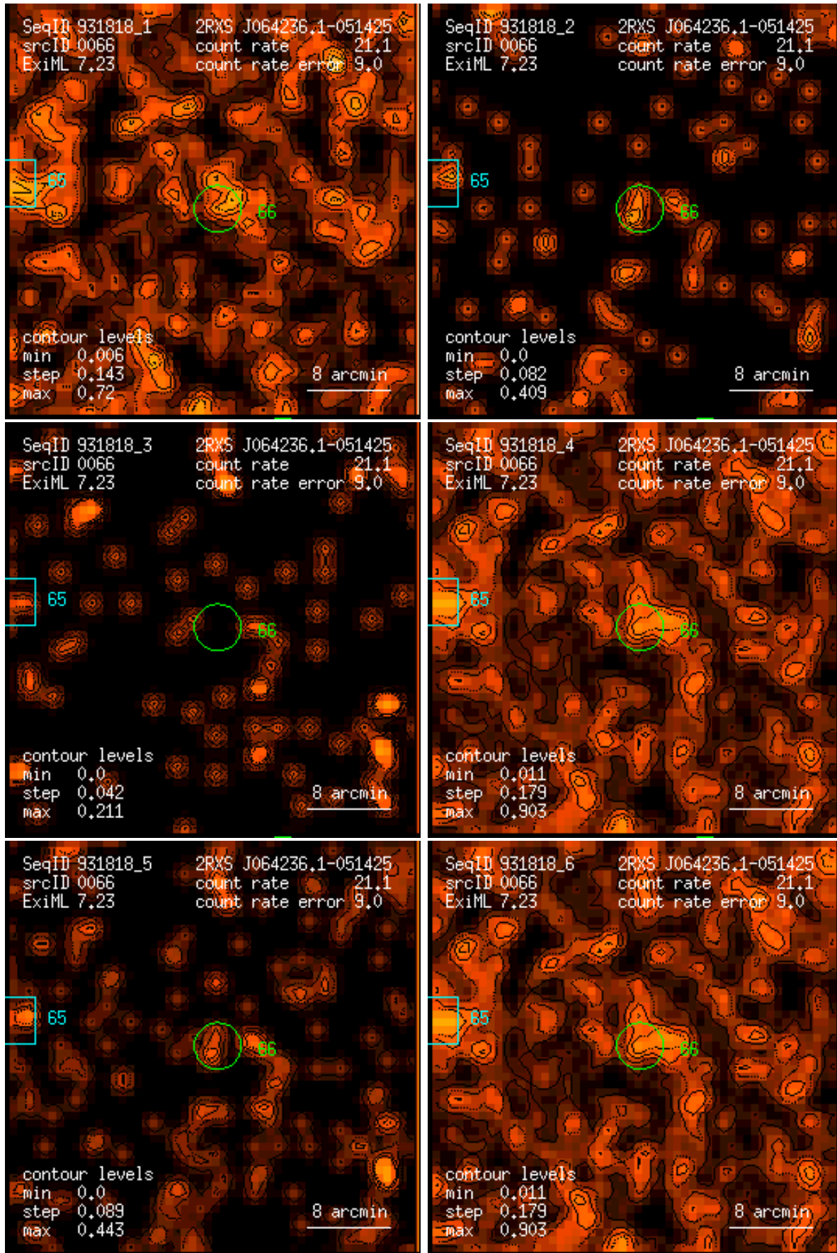
Figure 66: RASS 931818: detection 0066: band rate images, Gaussian filter: (1) PSPC channels 11 – 41, (2) 52 – 90, (3) 91 – 201, (4) 11 – 235, (5) 52 – 201, (6) 11 – 201. Broad band rates in counts/ks. Band rate contour levels in counts/ks/arcmin 2 .
