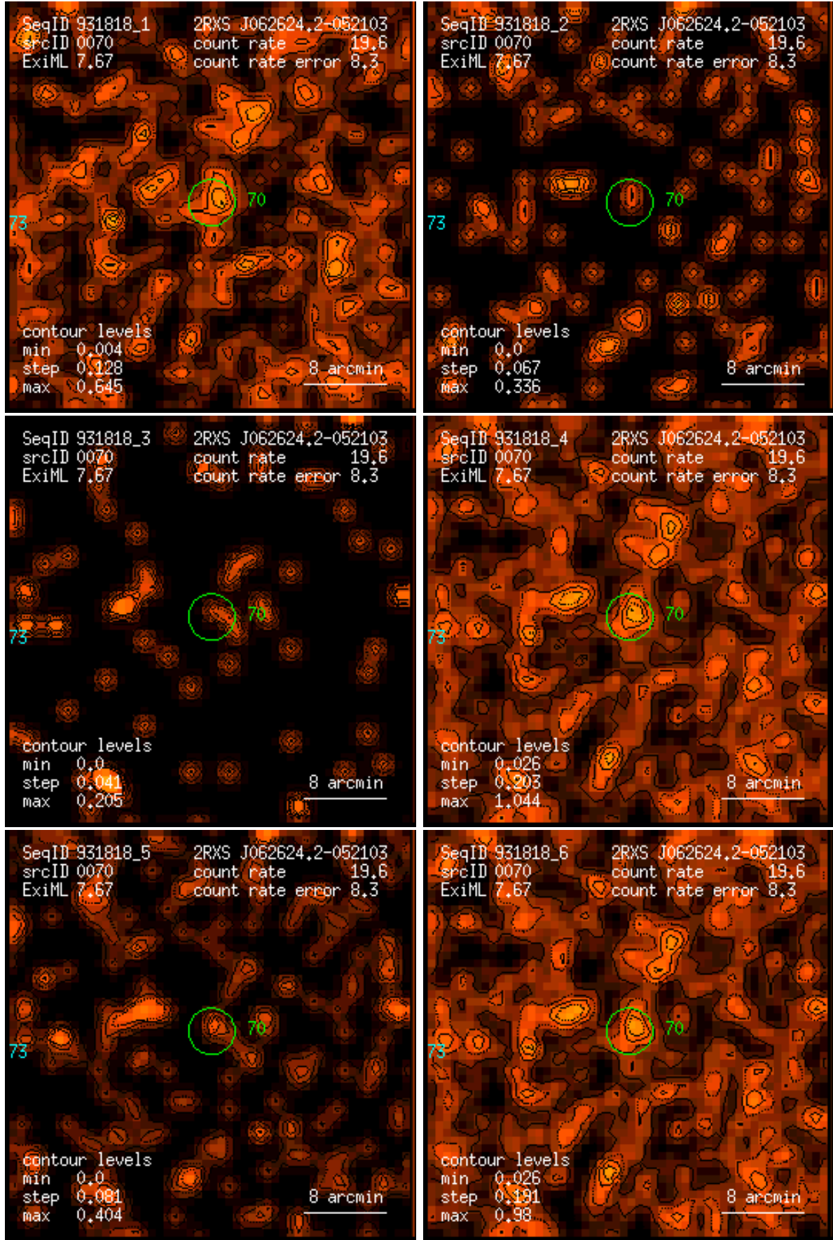
Figure 70: RASS 931818: detection 0070: band rate images, Gaussian filter: (1) PSPC channels 11 – 41, (2) 52 – 90, (3) 91 – 201, (4) 11 – 235, (5) 52 – 201, (6) 11 – 201. Broad band rates in counts/ks. Band rate contour levels in counts/ks/arcmin 2 .
