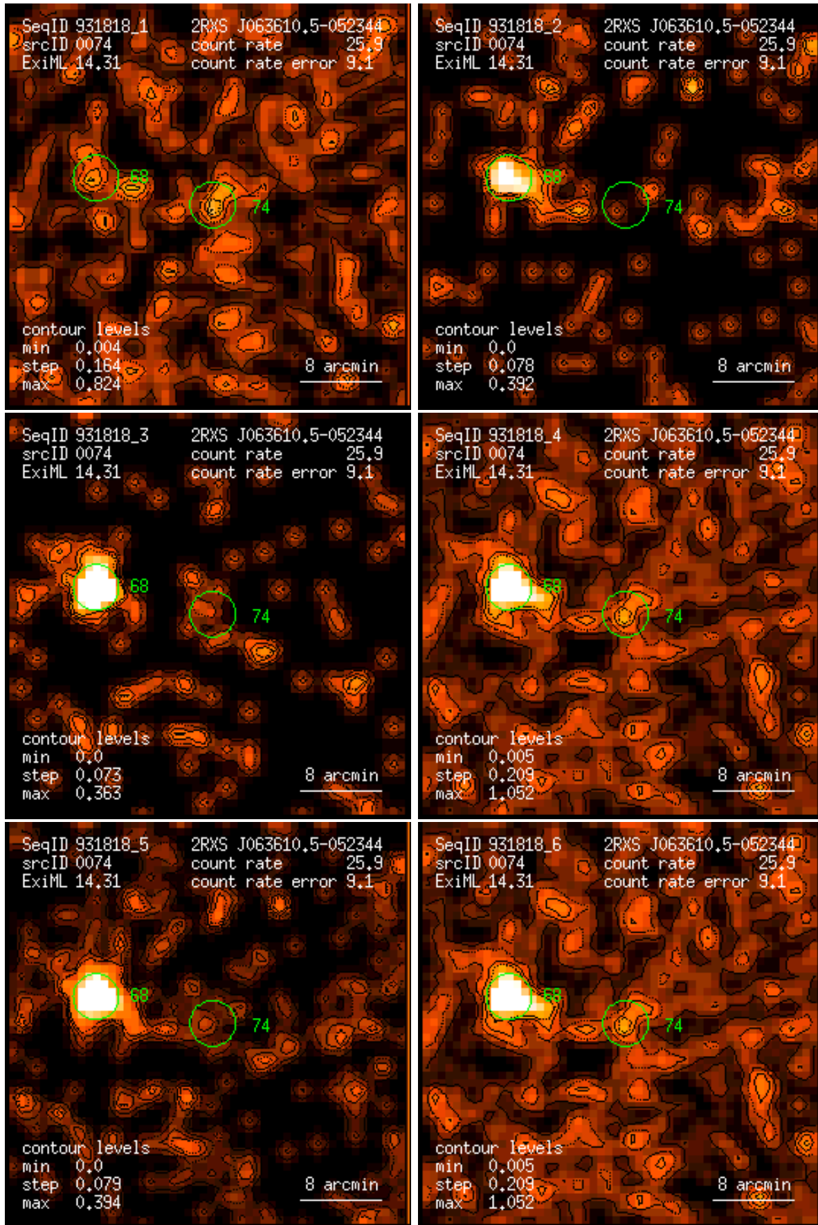
Figure 74: RASS 931818: detection 0074: band rate images, Gaussian filter: (1) PSPC channels 11 – 41, (2) 52 – 90, (3) 91 – 201, (4) 11 – 235, (5) 52 – 201, (6) 11 – 201. Broad band rates in counts/ks. Band rate contour levels in counts/ks/arcmin 2 .
