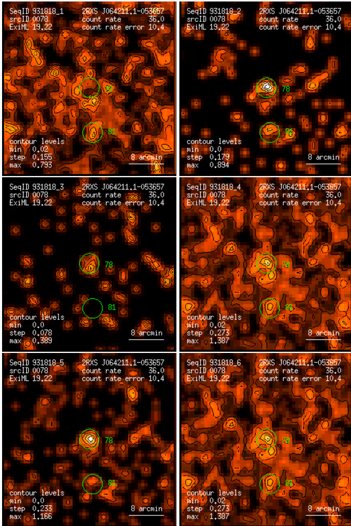
Figure 78: RASS 931818: detection 0078: band rate images, Gaussian filter: (1) PSPC channels 11 – 41, (2) 52 – 90, (3) 91 – 201, (4) 11 – 235, (5) 52 – 201, (6) 11 – 201. Broad band rates in counts/ks. Band rate contour levels in counts/ks/arcmin 2 .
