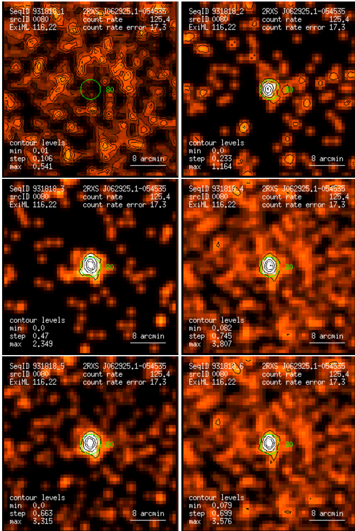
Figure 80: RASS 931818: detection 0080: band rate images, Gaussian filter: (1) PSPC channels 11 – 41, (2) 52 – 90, (3) 91 – 201, (4) 11 – 235, (5) 52 – 201, (6) 11 – 201. Broad band rates in counts/ks. Band rate contour levels in counts/ks/arcmin 2 .
