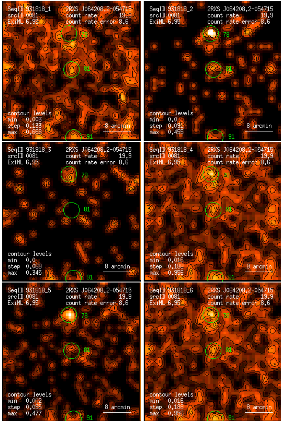
Figure 81: RASS 931818: detection 0081: band rate images, Gaussian filter: (1) PSPC channels 11 – 41, (2) 52 – 90, (3) 91 – 201, (4) 11 – 235, (5) 52 – 201, (6) 11 – 201. Broad band rates in counts/ks. Band rate contour levels in counts/ks/arcmin 2 .
