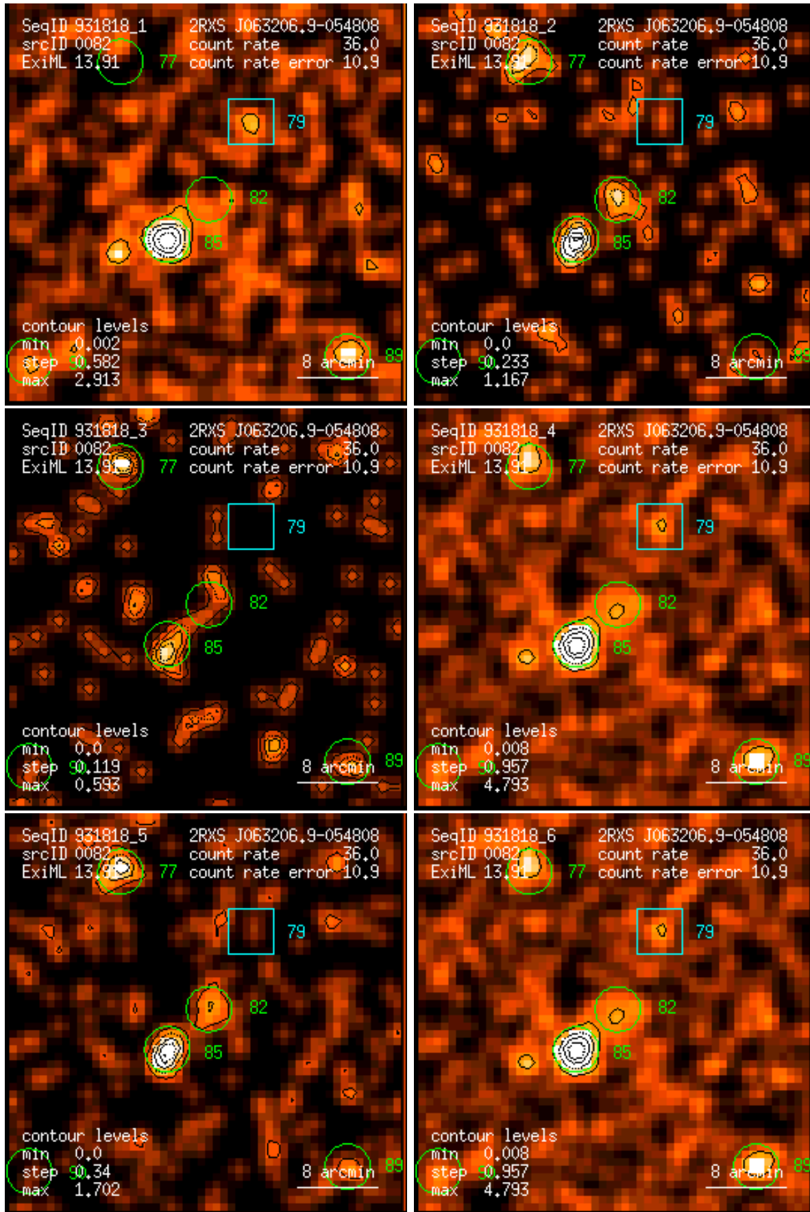
Figure 82: RASS 931818: detection 0082: band rate images, Gaussian filter: (1) PSPC channels 11 – 41, (2) 52 – 90, (3) 91 – 201, (4) 11 – 235, (5) 52 – 201, (6) 11 – 201. Broad band rates in counts/ks. Band rate contour levels in counts/ks/arcmin 2 .
