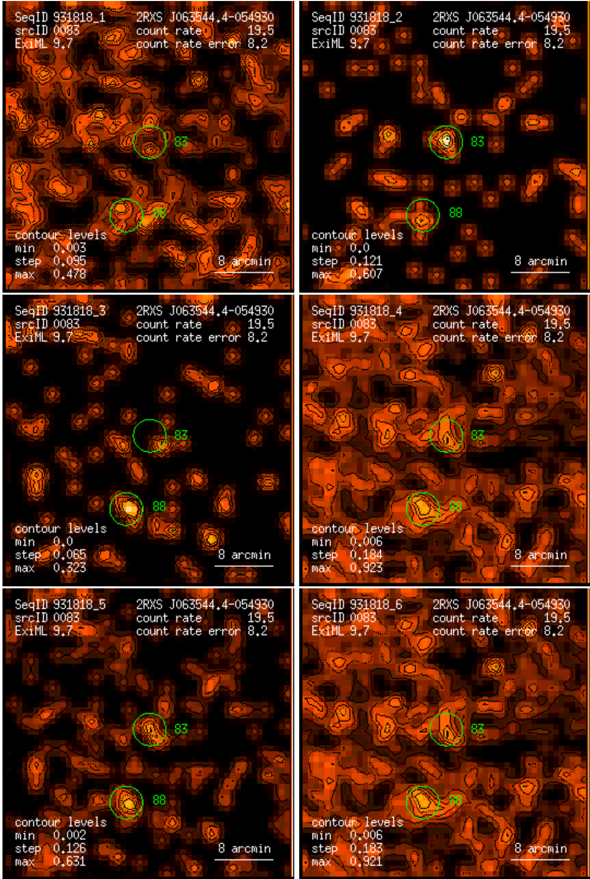
Figure 83: RASS 931818: detection 0083: band rate images, Gaussian filter: (1) PSPC channels 11 – 41, (2) 52 – 90, (3) 91 – 201, (4) 11 – 235, (5) 52 – 201, (6) 11 – 201. Broad band rates in counts/ks. Band rate contour levels in counts/ks/arcmin 2 .
