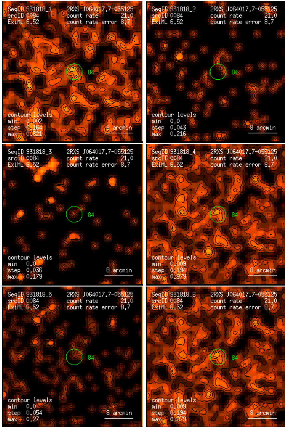
Figure 84: RASS 931818: detection 0084: band rate images, Gaussian filter: (1) PSPC channels 11 – 41, (2) 52 – 90, (3) 91 – 201, (4) 11 – 235, (5) 52 – 201, (6) 11 – 201. Broad band rates in counts/ks. Band rate contour levels in counts/ks/arcmin 2 .
