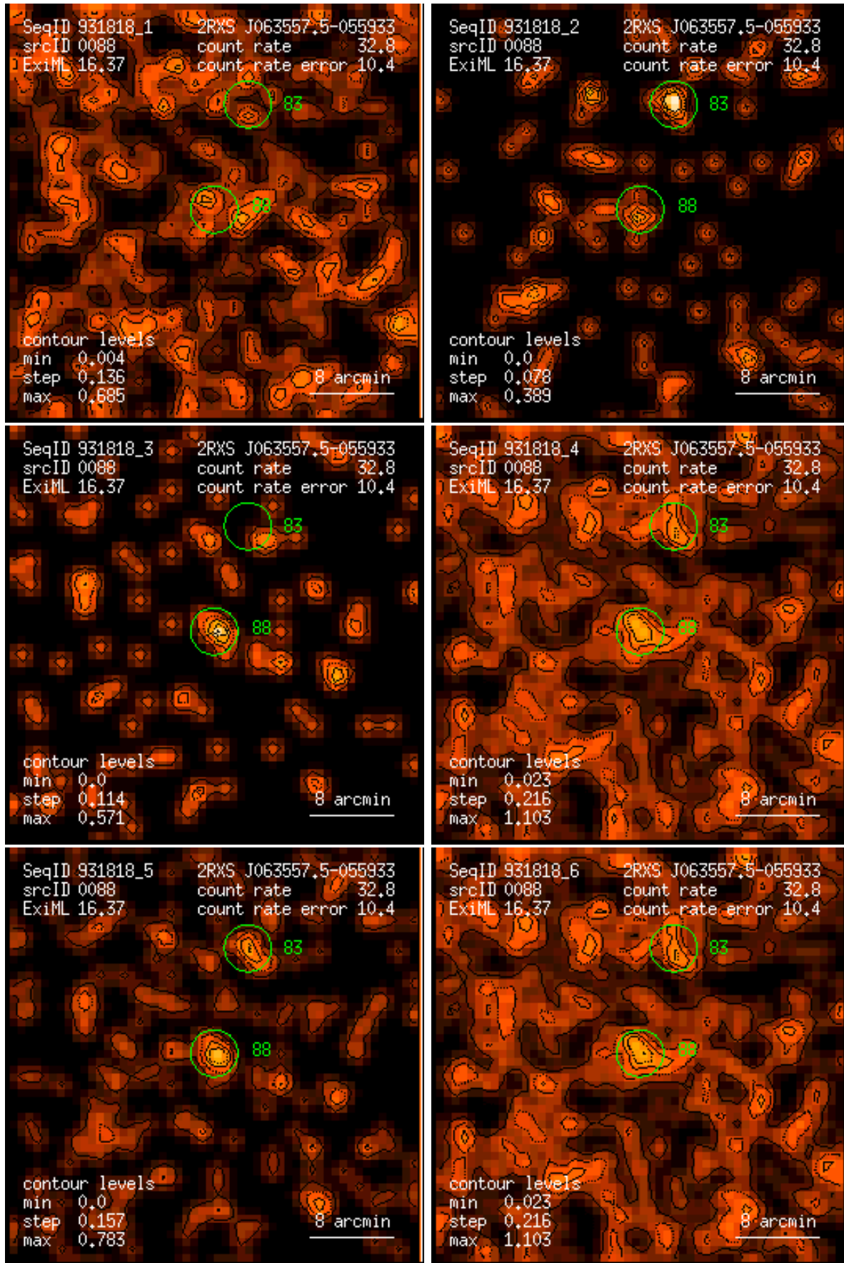
Figure 88: RASS 931818: detection 0088: band rate images, Gaussian filter: (1) PSPC channels 11 – 41, (2) 52 – 90, (3) 91 – 201, (4) 11 – 235, (5) 52 – 201, (6) 11 – 201. Broad band rates in counts/ks. Band rate contour levels in counts/ks/arcmin 2 .
