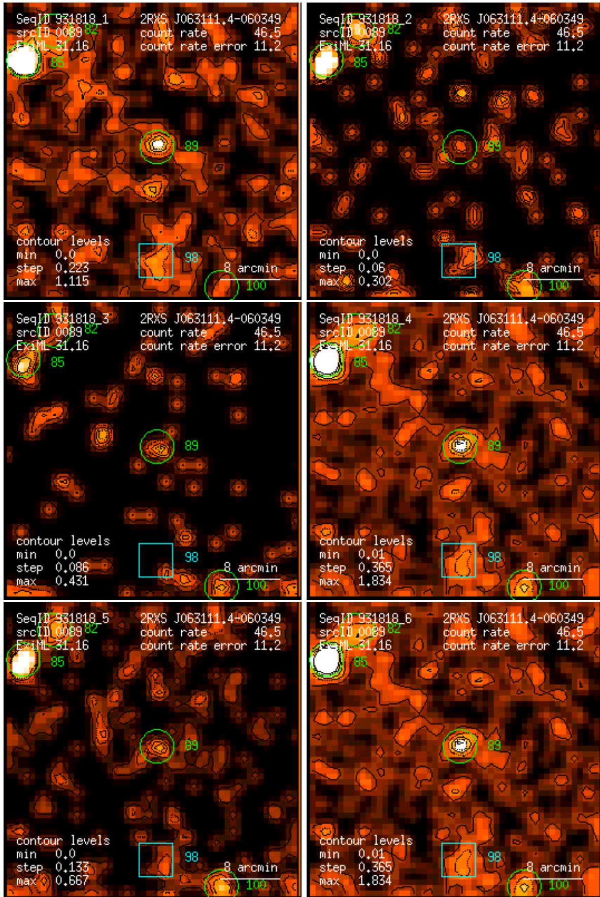
Figure 89: RASS 931818: detection 0089: band rate images, Gaussian filter: (1) PSPC channels 11 – 41, (2) 52 – 90, (3) 91 – 201, (4) 11 – 235, (5) 52 – 201, (6) 11 – 201. Broad band rates in counts/ks. Band rate contour levels in counts/ks/arcmin 2 .
