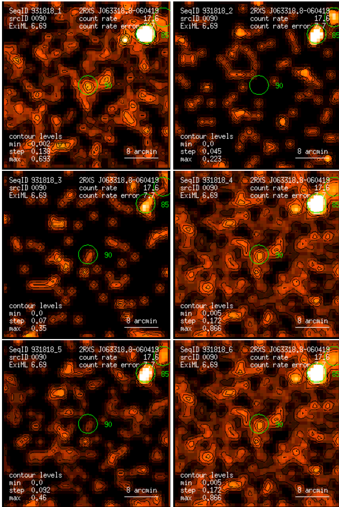
Figure 90: RASS 931818: detection 0090: band rate images, Gaussian filter: (1) PSPC channels 11 – 41, (2) 52 – 90, (3) 91 – 201, (4) 11 – 235, (5) 52 – 201, (6) 11 – 201. Broad band rates in counts/ks. Band rate contour levels in counts/ks/arcmin 2 .
