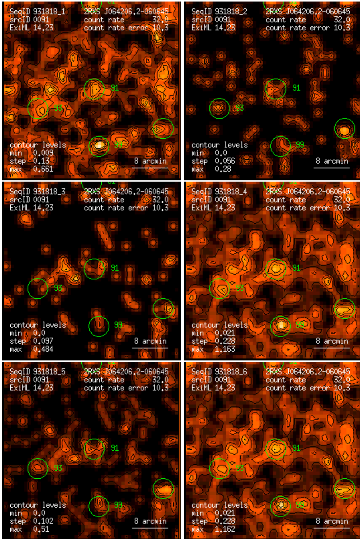
Figure 91: RASS 931818: detection 0091: band rate images, Gaussian filter: (1) PSPC channels 11 – 41, (2) 52 – 90, (3) 91 – 201, (4) 11 – 235, (5) 52 – 201, (6) 11 – 201. Broad band rates in counts/ks. Band rate contour levels in counts/ks/arcmin 2 .
