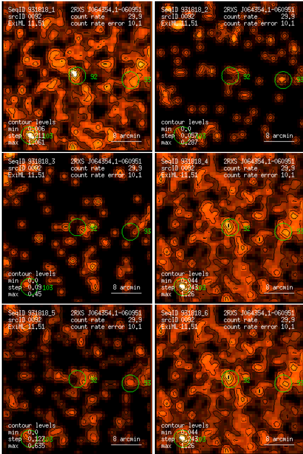
Figure 92: RASS 931818: detection 0092: band rate images, Gaussian filter: (1) PSPC channels 11 – 41, (2) 52 – 90, (3) 91 – 201, (4) 11 – 235, (5) 52 – 201, (6) 11 – 201. Broad band rates in counts/ks. Band rate contour levels in counts/ks/arcmin 2 .
