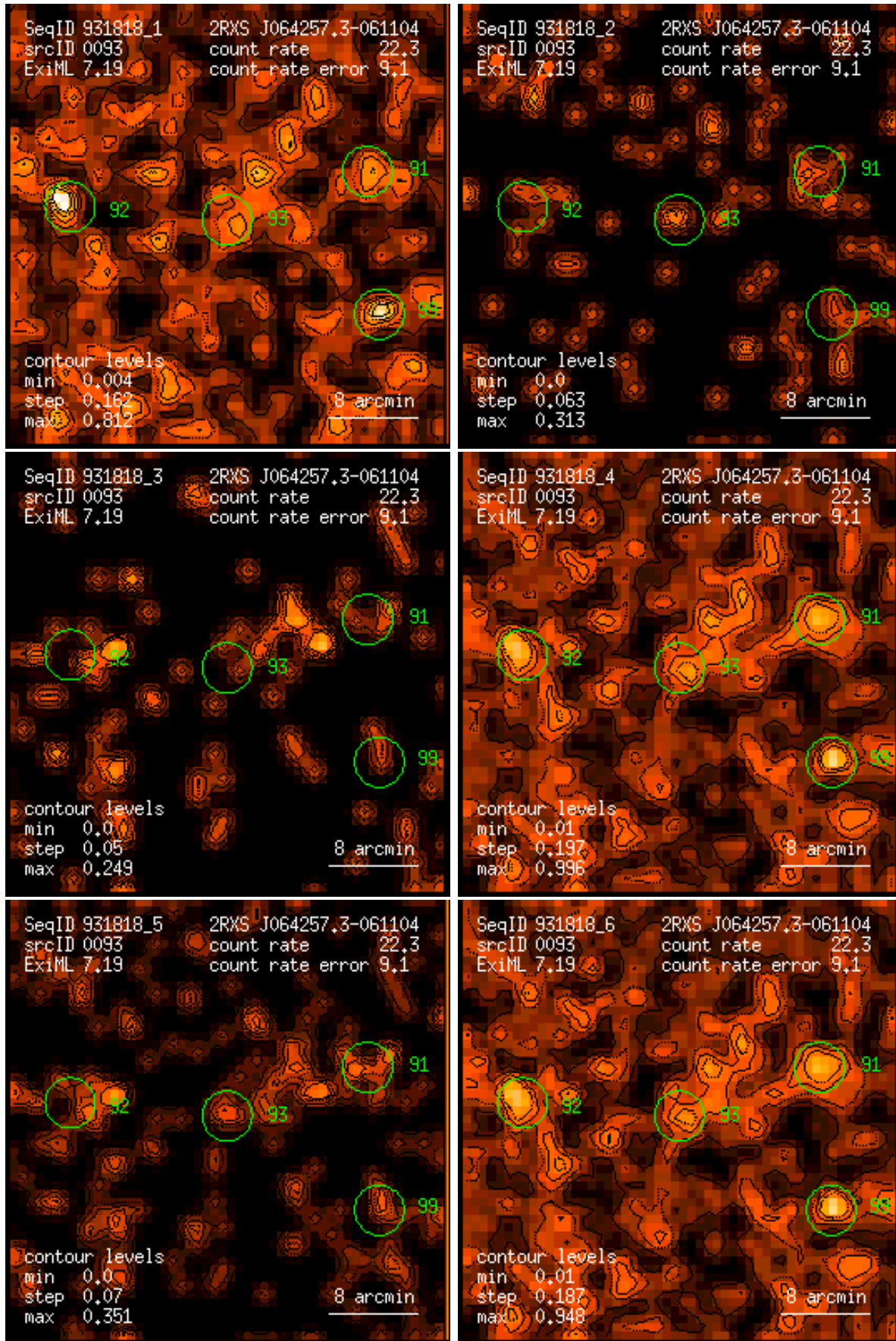
Figure 93: RASS 931818: detection 0093: band rate images, Gaussian filter: (1) PSPC channels 11 – 41, (2) 52 – 90, (3) 91 – 201, (4) 11 – 235, (5) 52 – 201, (6) 11 – 201. Broad band rates in counts/ks. Band rate contour levels in counts/ks/arcmin 2 .
