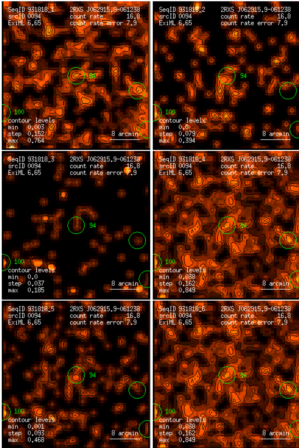
Figure 94: RASS 931818: detection 0094: band rate images, Gaussian filter: (1) PSPC channels 11 – 41, (2) 52 – 90, (3) 91 – 201, (4) 11 – 235, (5) 52 – 201, (6) 11 – 201. Broad band rates in counts/ks. Band rate contour levels in counts/ks/arcmin 2 .
