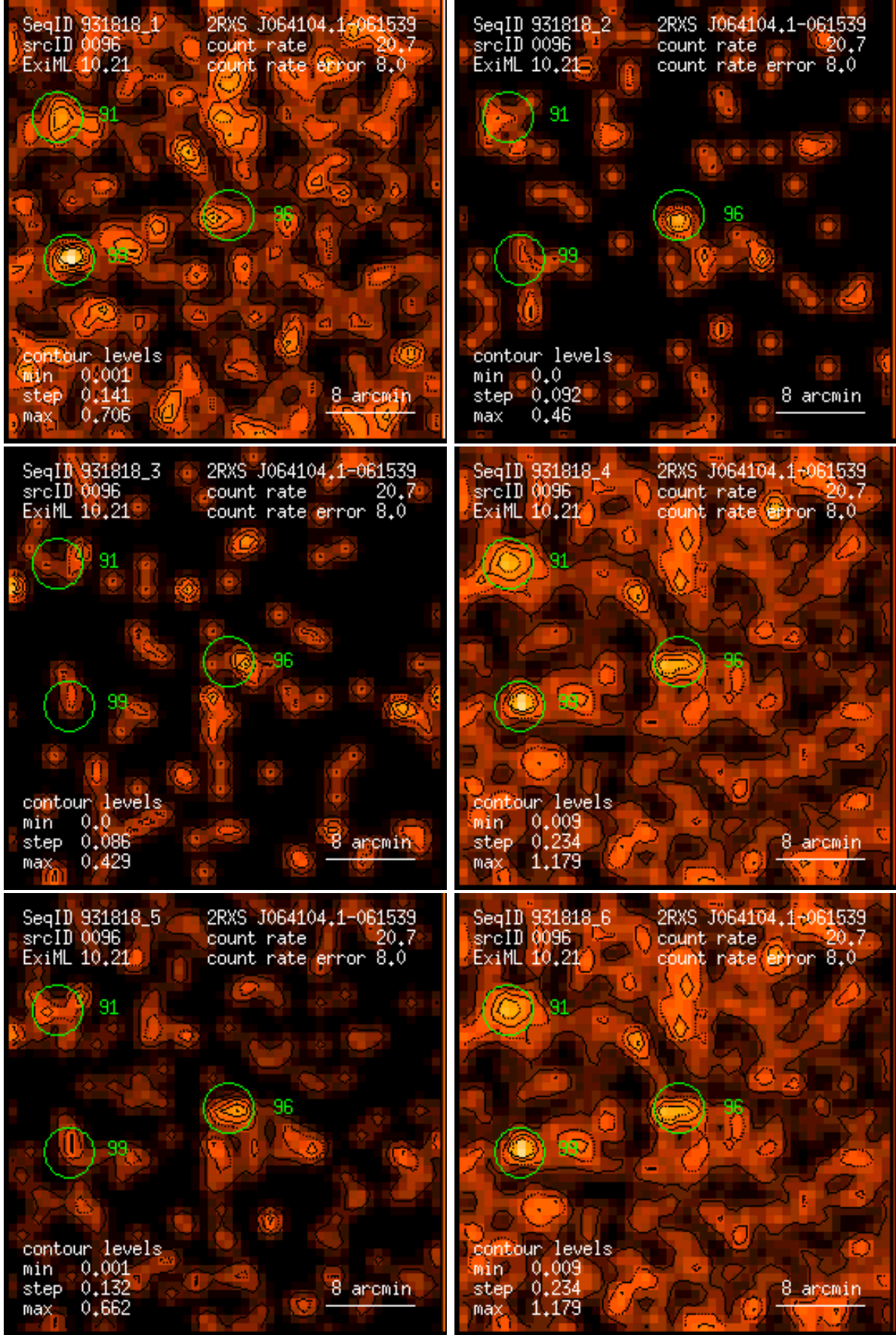
Figure 96: RASS 931818: detection 0096: band rate images, Gaussian filter: (1) PSPC channels 11 – 41, (2) 52 – 90, (3) 91 – 201, (4) 11 – 235, (5) 52 – 201, (6) 11 – 201. Broad band rates in counts/ks. Band rate contour levels in counts/ks/arcmin 2 .
