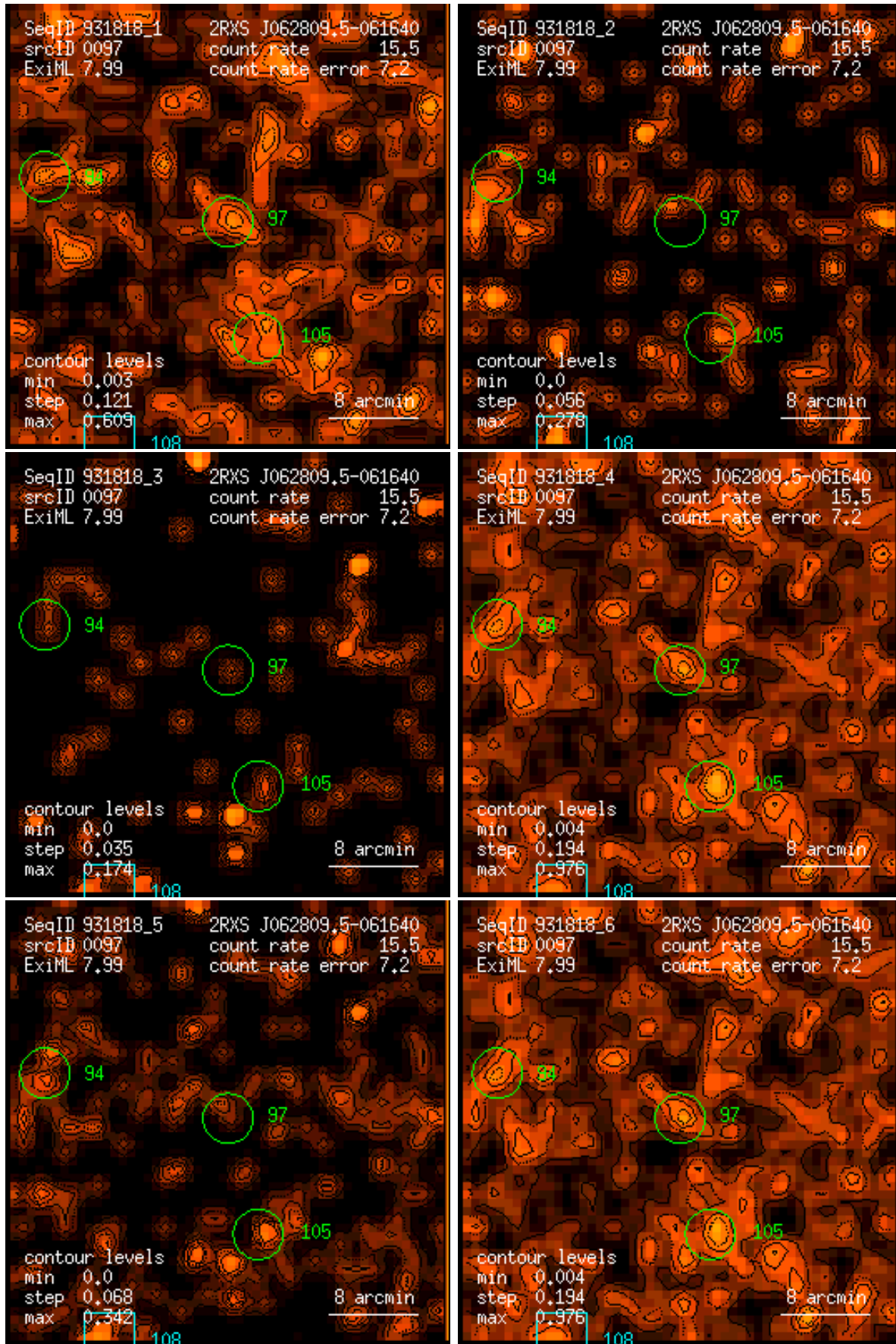
Figure 97: RASS 931818: detection 0097: band rate images, Gaussian filter: (1) PSPC channels 11 – 41, (2) 52 – 90, (3) 91 – 201, (4) 11 – 235, (5) 52 – 201, (6) 11 – 201. Broad band rates in counts/ks. Band rate contour levels in counts/ks/arcmin 2 .
