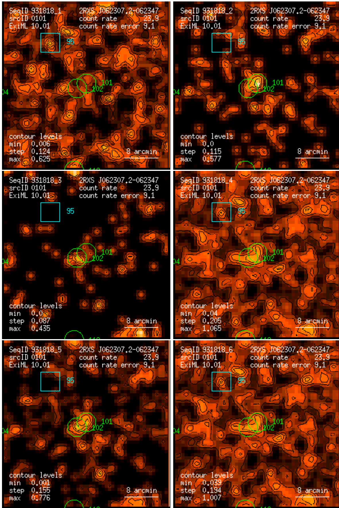
Figure 101: RASS 931818: detection 0101: band rate images, Gaussian filter: (1) PSPC channels 11 – 41, (2) 52 – 90, (3) 91 – 201, (4) 11 – 235, (5) 52 – 201, (6) 11 – 201. Broad band rates in counts/ks. Band rate contour levels in counts/ks/arcmin 2 .
