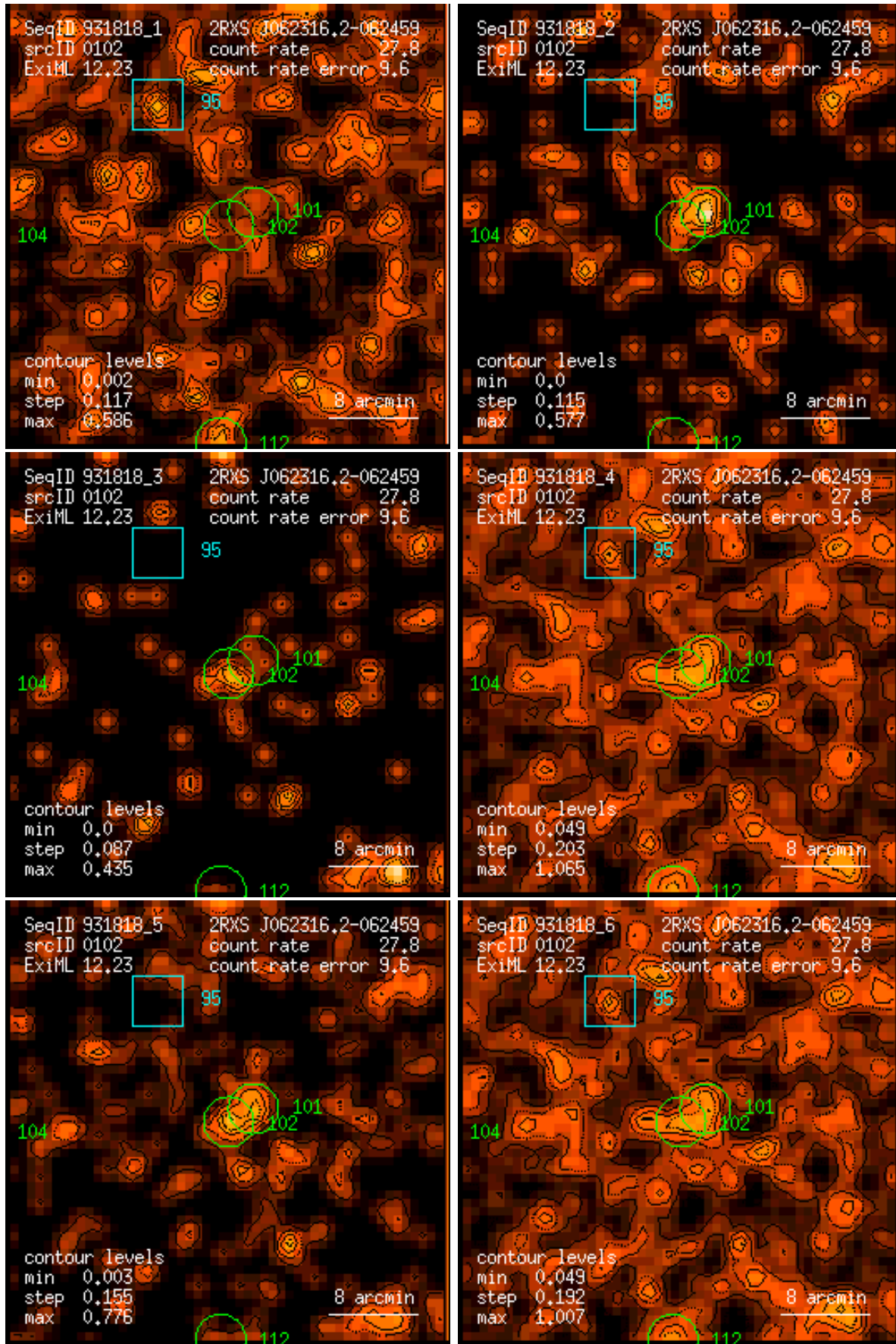
Figure 102: RASS 931818: detection 0102: band rate images, Gaussian filter: (1) PSPC channels 11 – 41, (2) 52 – 90, (3) 91 – 201, (4) 11 – 235, (5) 52 – 201, (6) 11 – 201. Broad band rates in counts/ks. Band rate contour levels in counts/ks/arcmin 2 .
