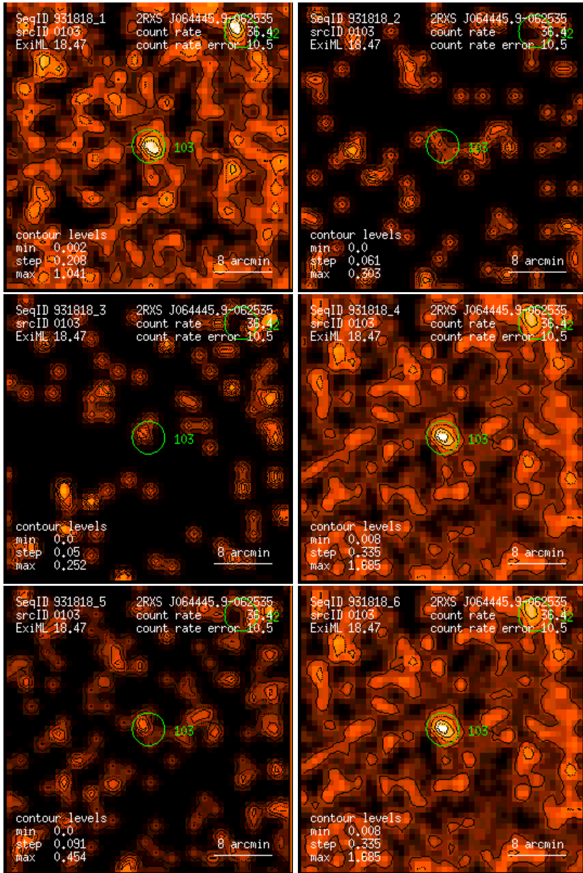
Figure 103: RASS 931818: detection 0103: band rate images, Gaussian filter: (1) PSPC channels 11 – 41, (2) 52 – 90, (3) 91 – 201, (4) 11 – 235, (5) 52 – 201, (6) 11 – 201. Broad band rates in counts/ks. Band rate contour levels in counts/ks/arcmin 2 .
