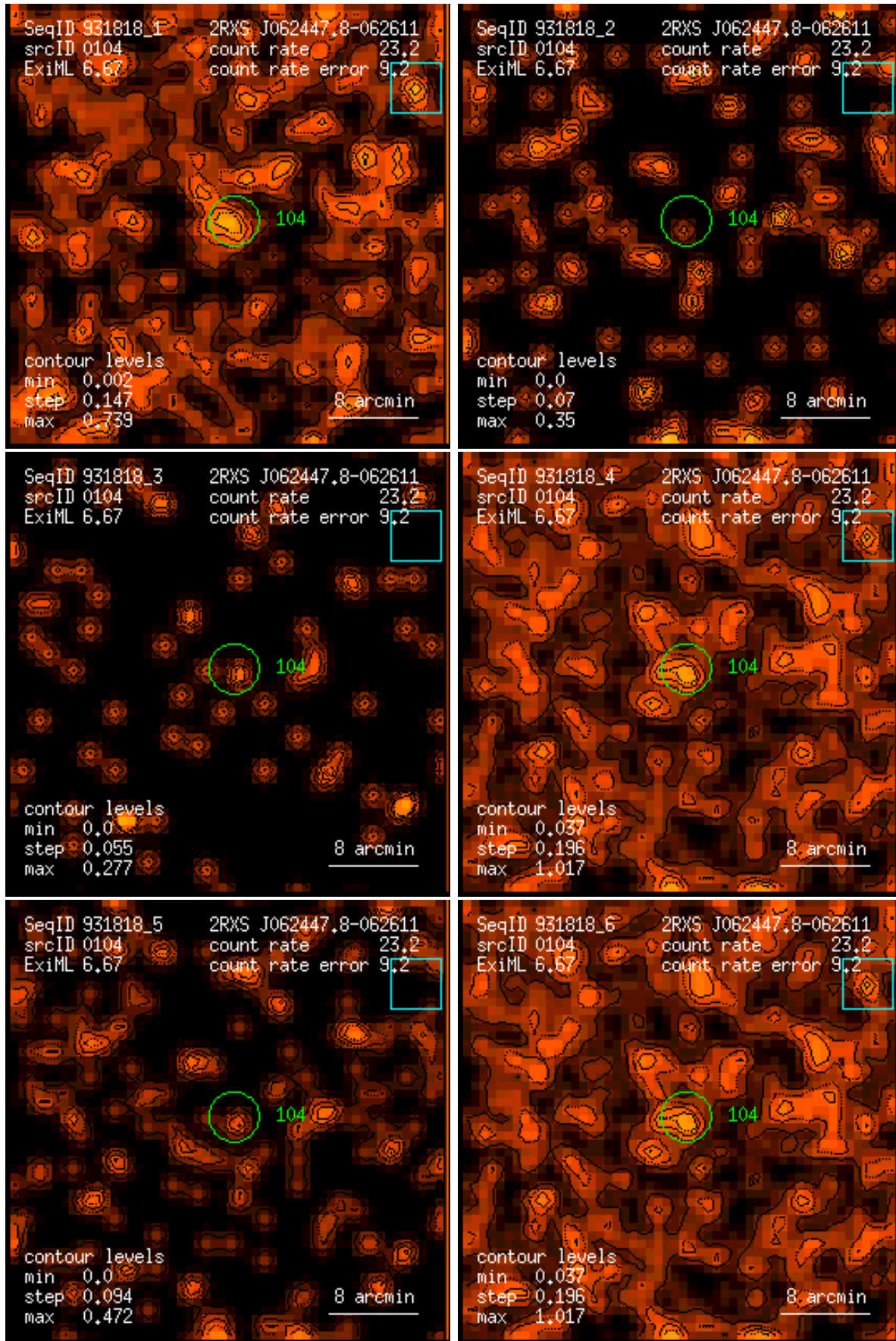
Figure 104: RASS 931818: detection 0104: band rate images, Gaussian filter: (1) PSPC channels 11 – 41, (2) 52 – 90, (3) 91 – 201, (4) 11 – 235, (5) 52 – 201, (6) 11 – 201. Broad band rates in counts/ks. Band rate contour levels in counts/ks/arcmin 2 .
