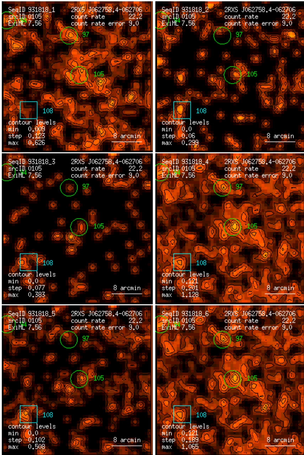
Figure 105: RASS 931818: detection 0105: band rate images, Gaussian filter: (1) PSPC channels 11 – 41, (2) 52 – 90, (3) 91 – 201, (4) 11 – 235, (5) 52 – 201, (6) 11 – 201. Broad band rates in counts/ks. Band rate contour levels in counts/ks/arcmin 2 .
