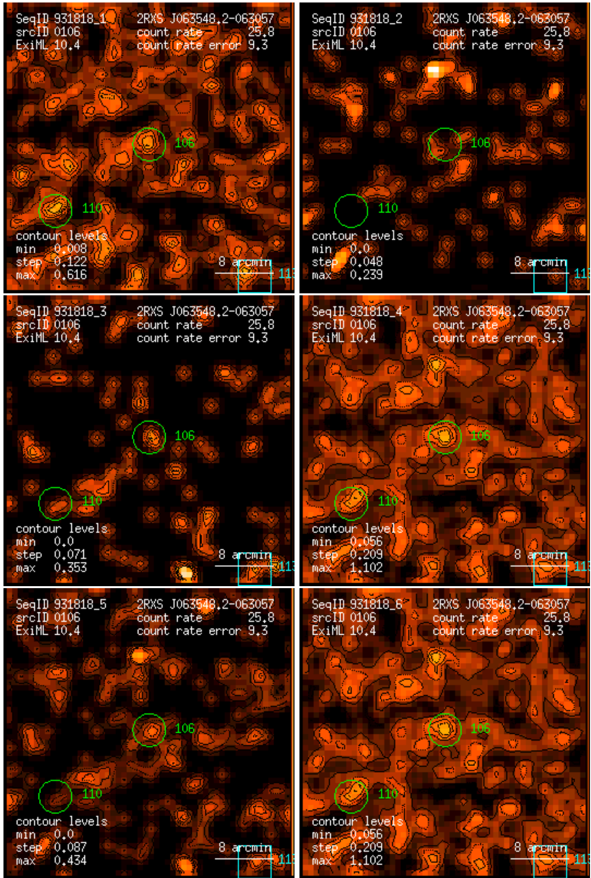
Figure 106: RASS 931818: detection 0106: band rate images, Gaussian filter: (1) PSPC channels 11 – 41, (2) 52 – 90, (3) 91 – 201, (4) 11 – 235, (5) 52 – 201, (6) 11 – 201. Broad band rates in counts/ks. Band rate contour levels in counts/ks/arcmin 2 .
