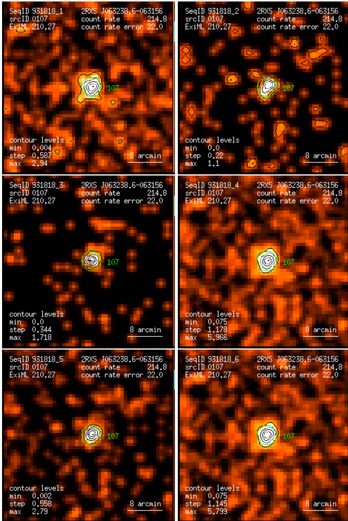
Figure 107: RASS 931818: detection 0107: band rate images, Gaussian filter: (1) PSPC channels 11 – 41, (2) 52 – 90, (3) 91 – 201, (4) 11 – 235, (5) 52 – 201, (6) 11 – 201. Broad band rates in counts/ks. Band rate contour levels in counts/ks/arcmin 2 .
