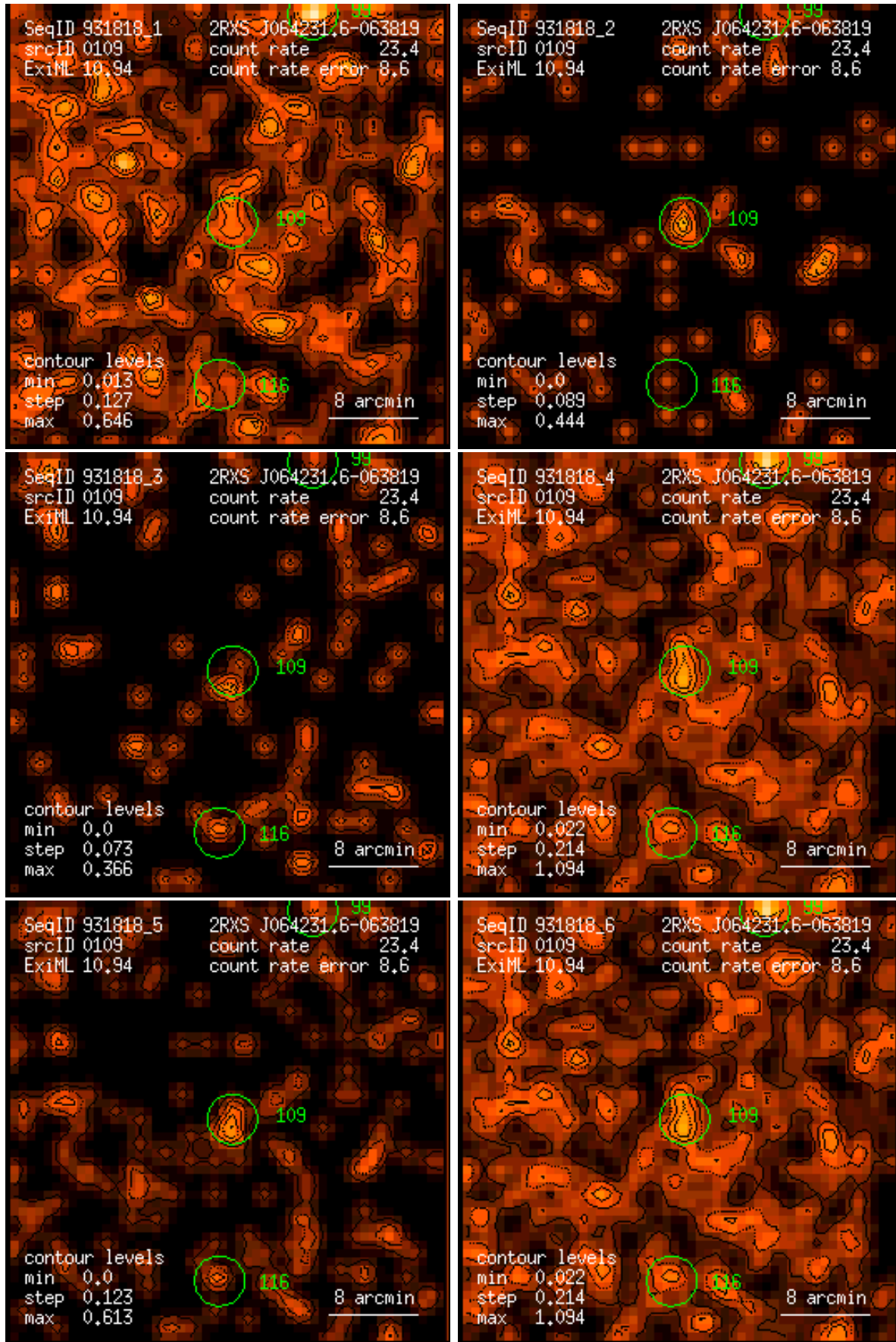
Figure 109: RASS 931818: detection 0109: band rate images, Gaussian filter: (1) PSPC channels 11 – 41, (2) 52 – 90, (3) 91 – 201, (4) 11 – 235, (5) 52 – 201, (6) 11 – 201. Broad band rates in counts/ks. Band rate contour levels in counts/ks/arcmin 2 .
