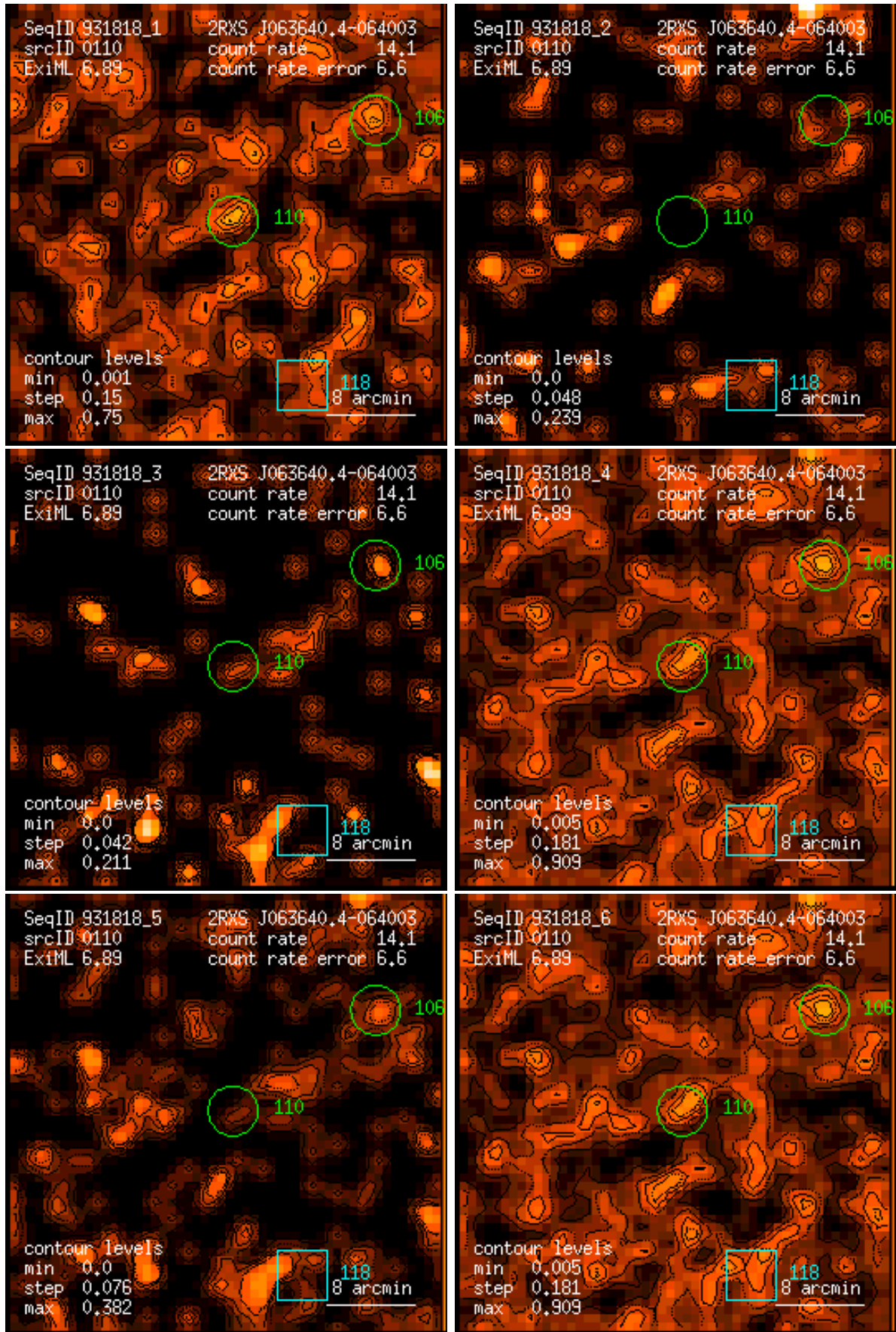
Figure 110: RASS 931818: detection 0110: band rate images, Gaussian filter: (1) PSPC channels 11 – 41, (2) 52 – 90, (3) 91 – 201, (4) 11 – 235, (5) 52 – 201, (6) 11 – 201. Broad band rates in counts/ks. Band rate contour levels in counts/ks/arcmin 2 .
