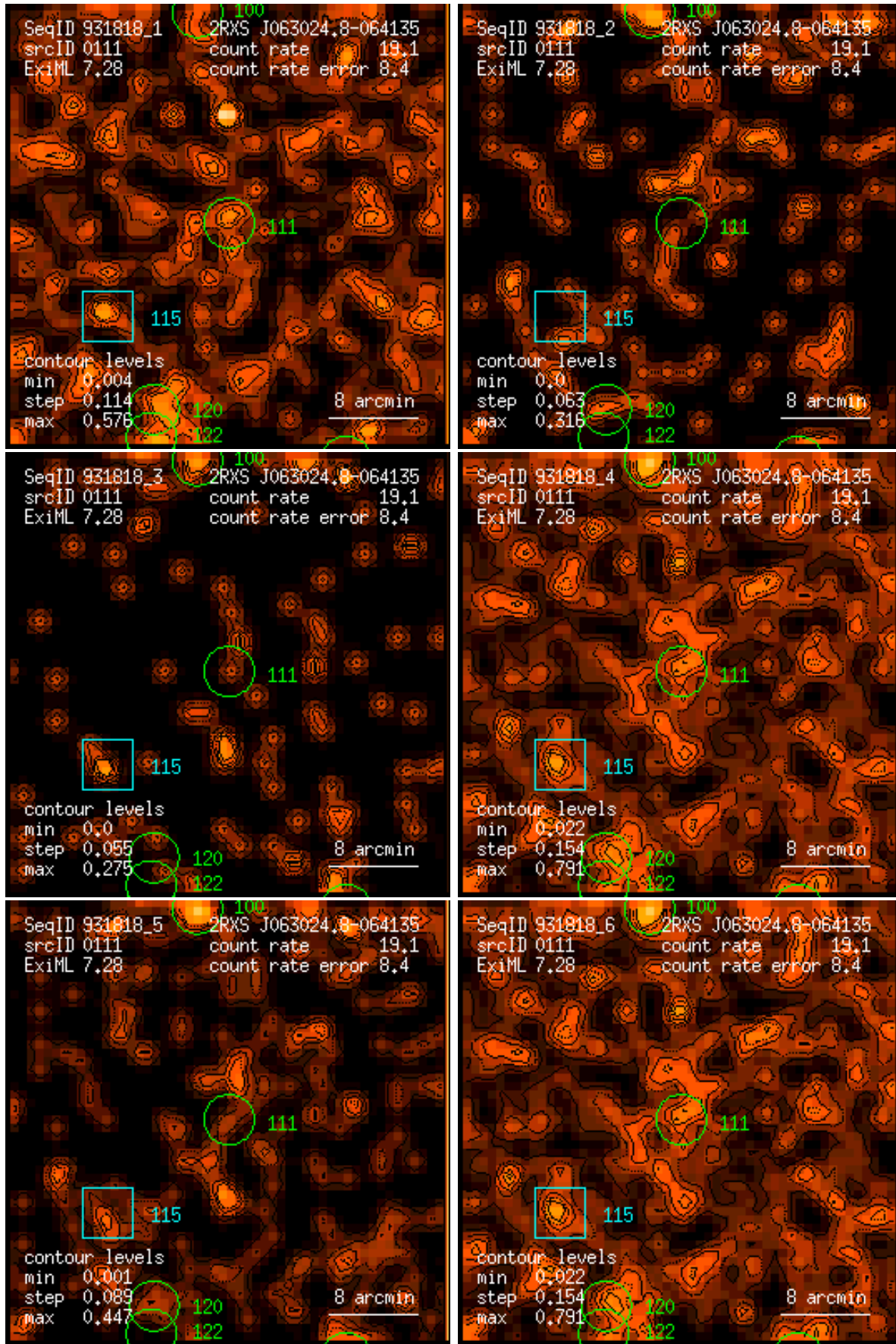
Figure 111: RASS 931818: detection 0111: band rate images, Gaussian filter: (1) PSPC channels 11 – 41, (2) 52 – 90, (3) 91 – 201, (4) 11 – 235, (5) 52 – 201, (6) 11 – 201. Broad band rates in counts/ks. Band rate contour levels in counts/ks/arcmin 2 .
