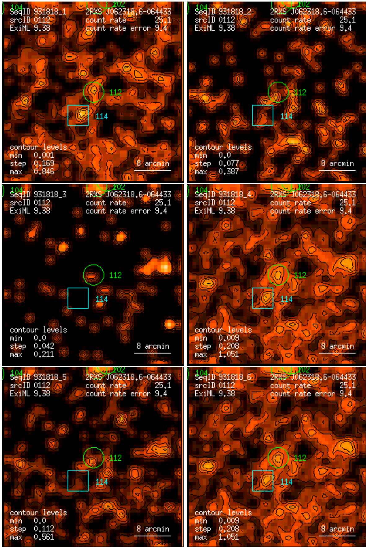
Figure 112: RASS 931818: detection 0112: band rate images, Gaussian filter: (1) PSPC channels 11 – 41, (2) 52 – 90, (3) 91 – 201, (4) 11 – 235, (5) 52 – 201, (6) 11 – 201. Broad band rates in counts/ks. Band rate contour levels in counts/ks/arcmin 2 .
