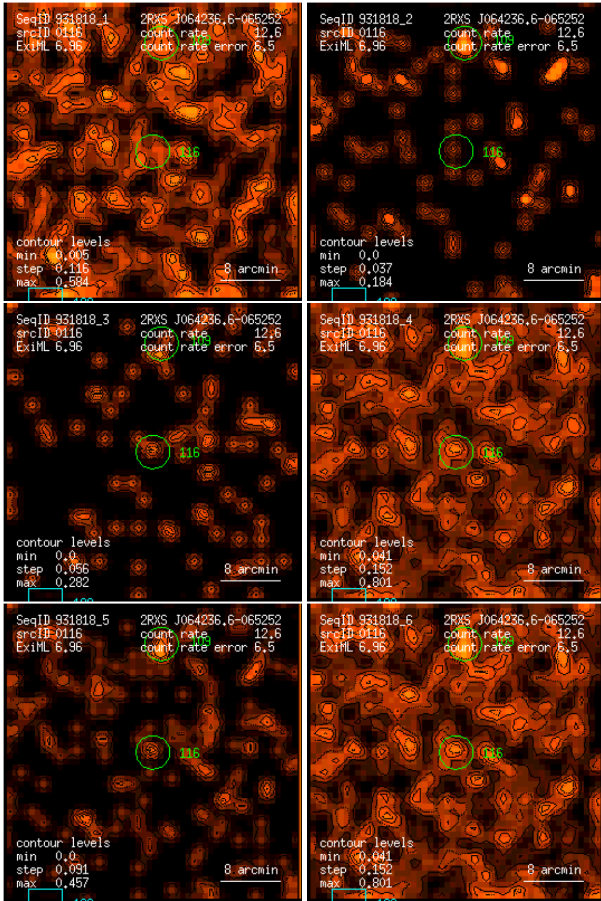
Figure 116: RASS 931818: detection 0116: band rate images, Gaussian filter: (1) PSPC channels 11 – 41, (2) 52 – 90, (3) 91 – 201, (4) 11 – 235, (5) 52 – 201, (6) 11 – 201. Broad band rates in counts/ks. Band rate contour levels in counts/ks/arcmin 2 .
