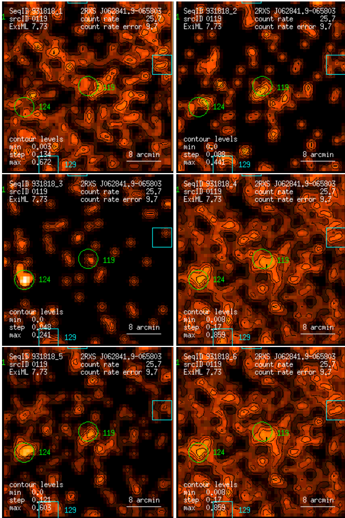
Figure 119: RASS 931818: detection 0119: band rate images, Gaussian filter: (1) PSPC channels 11 – 41, (2) 52 – 90, (3) 91 – 201, (4) 11 – 235, (5) 52 – 201, (6) 11 – 201. Broad band rates in counts/ks. Band rate contour levels in counts/ks/arcmin 2 .
