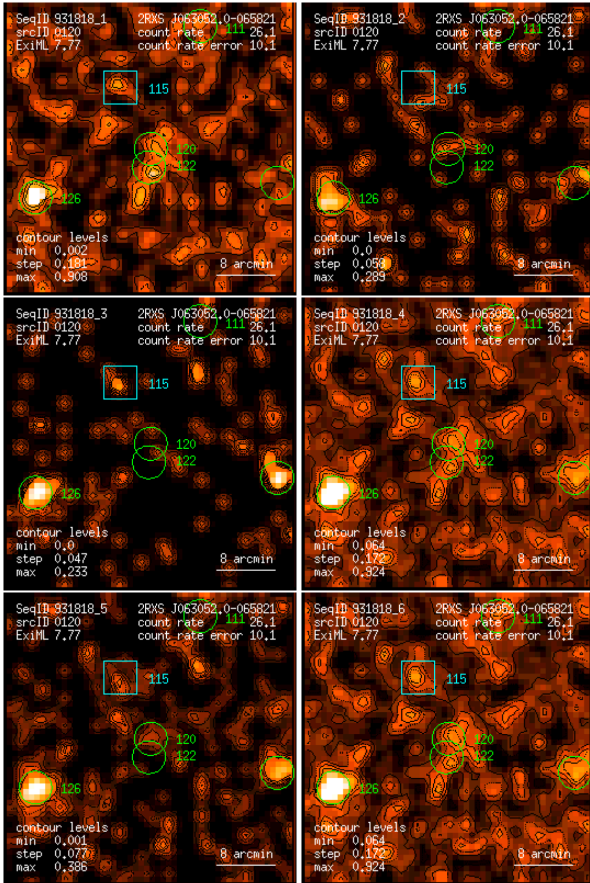
Figure 120: RASS 931818: detection 0120: band rate images, Gaussian filter: (1) PSPC channels 11 – 41, (2) 52 – 90, (3) 91 – 201, (4) 11 – 235, (5) 52 – 201, (6) 11 – 201. Broad band rates in counts/ks. Band rate contour levels in counts/ks/arcmin 2 .
