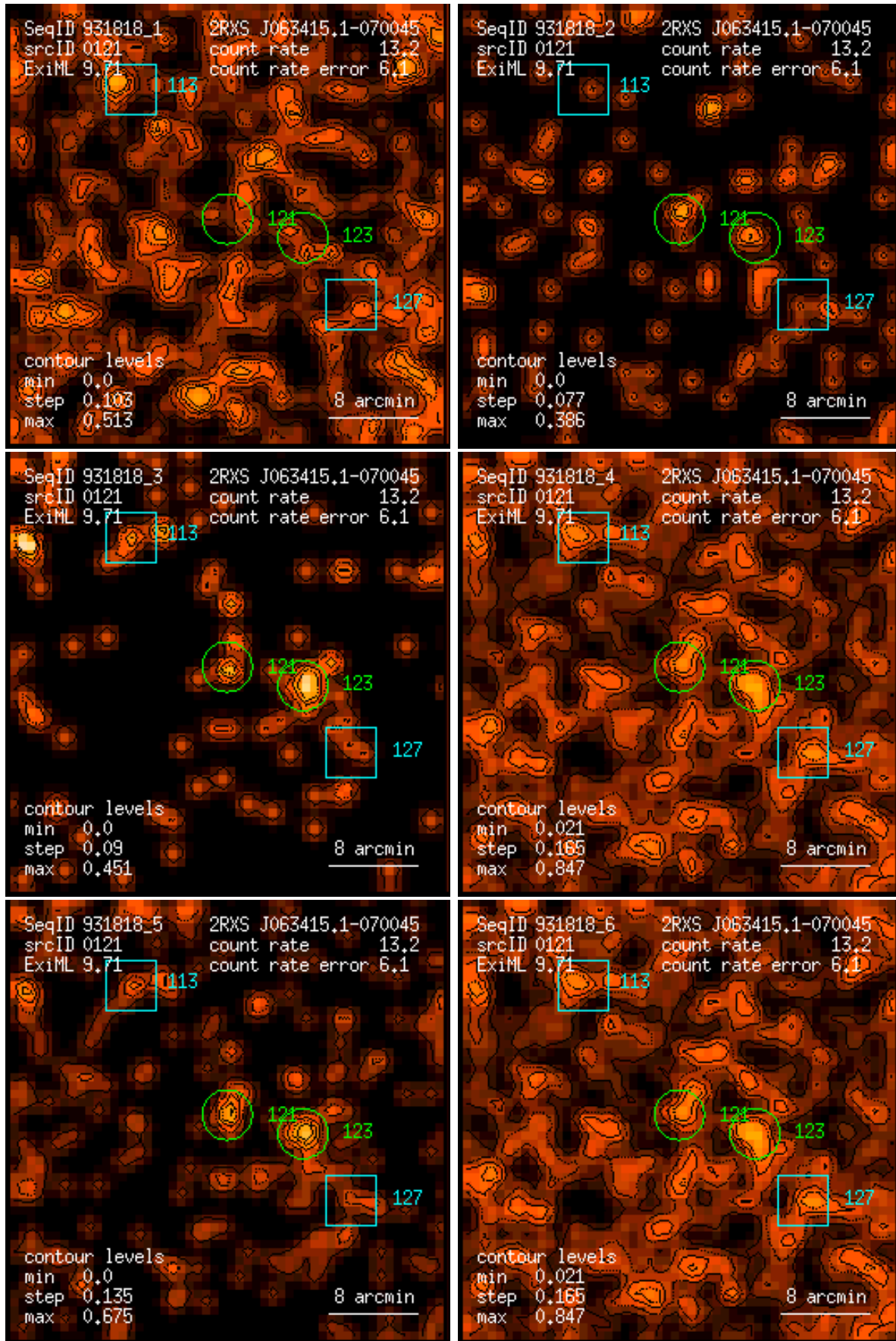
Figure 121: RASS 931818: detection 0121: band rate images, Gaussian filter: (1) PSPC channels 11 – 41, (2) 52 – 90, (3) 91 – 201, (4) 11 – 235, (5) 52 – 201, (6) 11 – 201. Broad band rates in counts/ks. Band rate contour levels in counts/ks/arcmin 2 .
