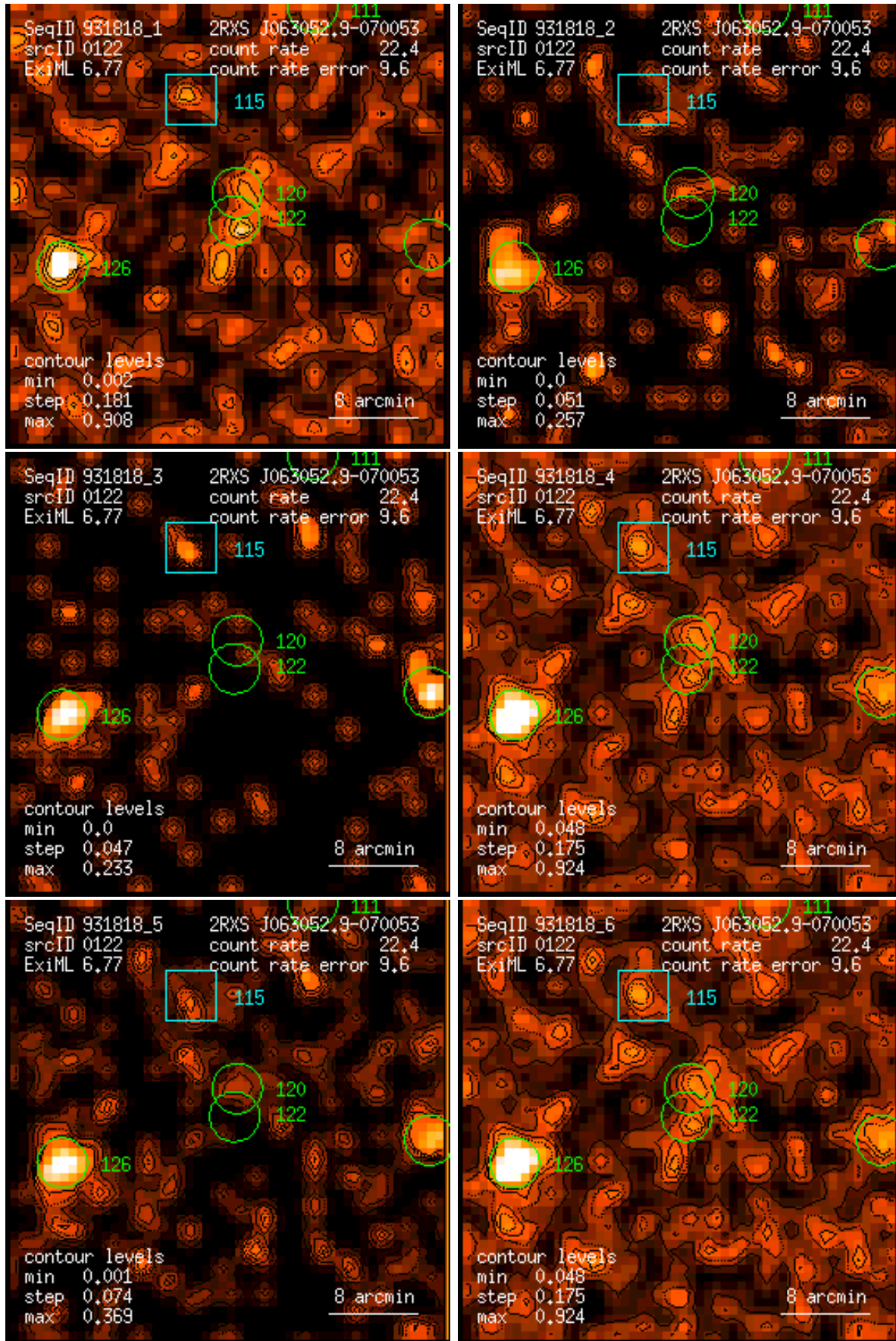
Figure 122: RASS 931818: detection 0122: band rate images, Gaussian filter: (1) PSPC channels 11 – 41, (2) 52 – 90, (3) 91 – 201, (4) 11 – 235, (5) 52 – 201, (6) 11 – 201. Broad band rates in counts/ks. Band rate contour levels in counts/ks/arcmin 2 .
