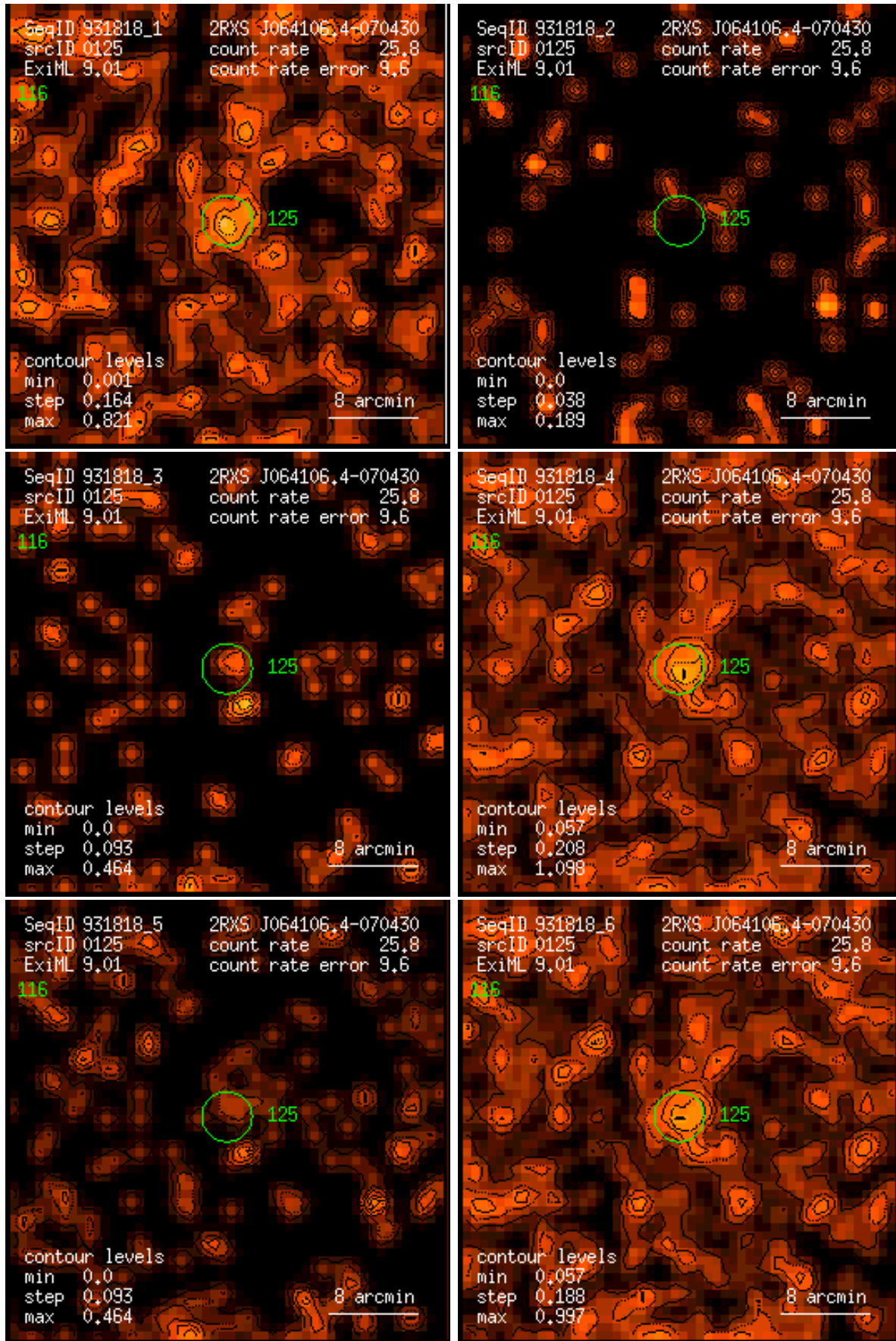
Figure 125: RASS 931818: detection 0125: band rate images, Gaussian filter: (1) PSPC channels 11 – 41, (2) 52 – 90, (3) 91 – 201, (4) 11 – 235, (5) 52 – 201, (6) 11 – 201. Broad band rates in counts/ks. Band rate contour levels in counts/ks/arcmin 2 .
