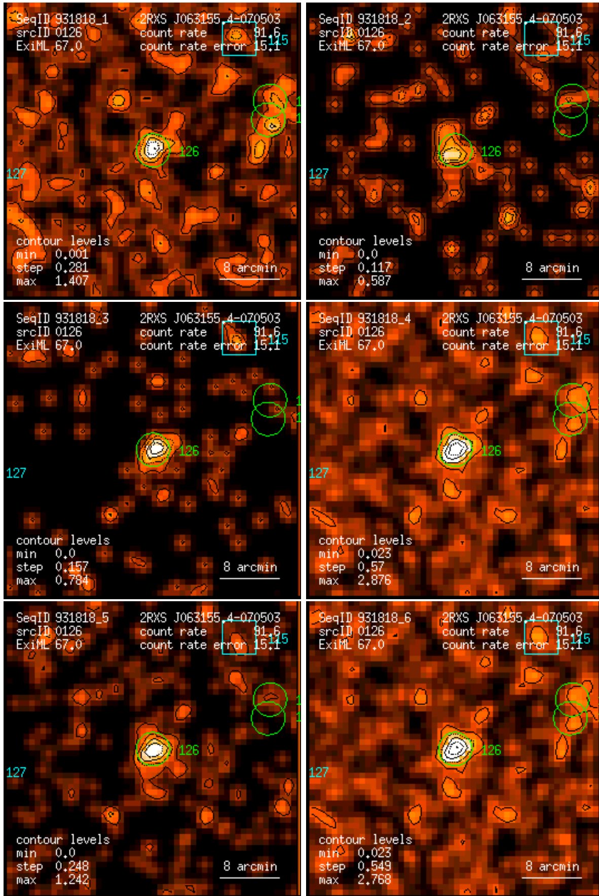
Figure 126: RASS 931818: detection 0126: band rate images, Gaussian filter: (1) PSPC channels 11 – 41, (2) 52 – 90, (3) 91 – 201, (4) 11 – 235, (5) 52 – 201, (6) 11 – 201. Broad band rates in counts/ks. Band rate contour levels in counts/ks/arcmin 2 .
