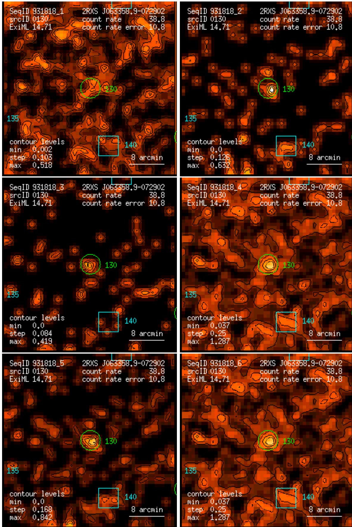
Figure 130: RASS 931818: detection 0130: band rate images, Gaussian filter: (1) PSPC channels 11 – 41, (2) 52 – 90, (3) 91 – 201, (4) 11 – 235, (5) 52 – 201, (6) 11 – 201. Broad band rates in counts/ks. Band rate contour levels in counts/ks/arcmin 2 .
