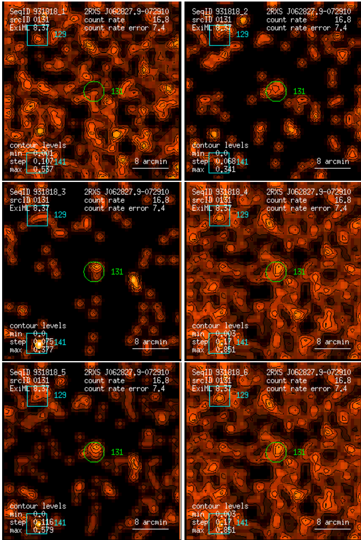
Figure 131: RASS 931818: detection 0131: band rate images, Gaussian filter: (1) PSPC channels 11 – 41, (2) 52 – 90, (3) 91 – 201, (4) 11 – 235, (5) 52 – 201, (6) 11 – 201. Broad band rates in counts/ks. Band rate contour levels in counts/ks/arcmin 2 .
