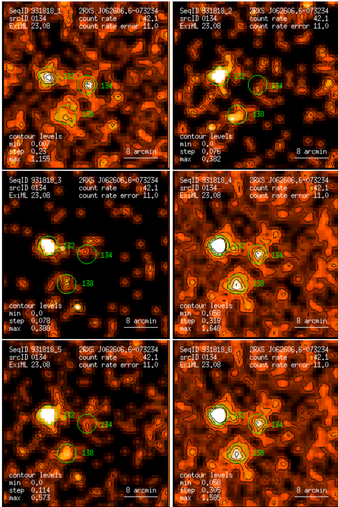
Figure 134: RASS 931818: detection 0134: band rate images, Gaussian filter: (1) PSPC channels 11 – 41, (2) 52 – 90, (3) 91 – 201, (4) 11 – 235, (5) 52 – 201, (6) 11 – 201. Broad band rates in counts/ks. Band rate contour levels in counts/ks/arcmin 2 .
