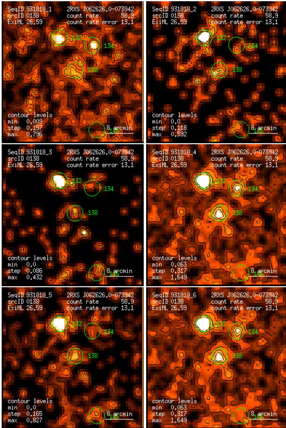
Figure 138: RASS 931818: detection 0138: band rate images, Gaussian filter: (1) PSPC channels 11 – 41, (2) 52 – 90, (3) 91 – 201, (4) 11 – 235, (5) 52 – 201, (6) 11 – 201. Broad band rates in counts/ks. Band rate contour levels in counts/ks/arcmin 2 .
