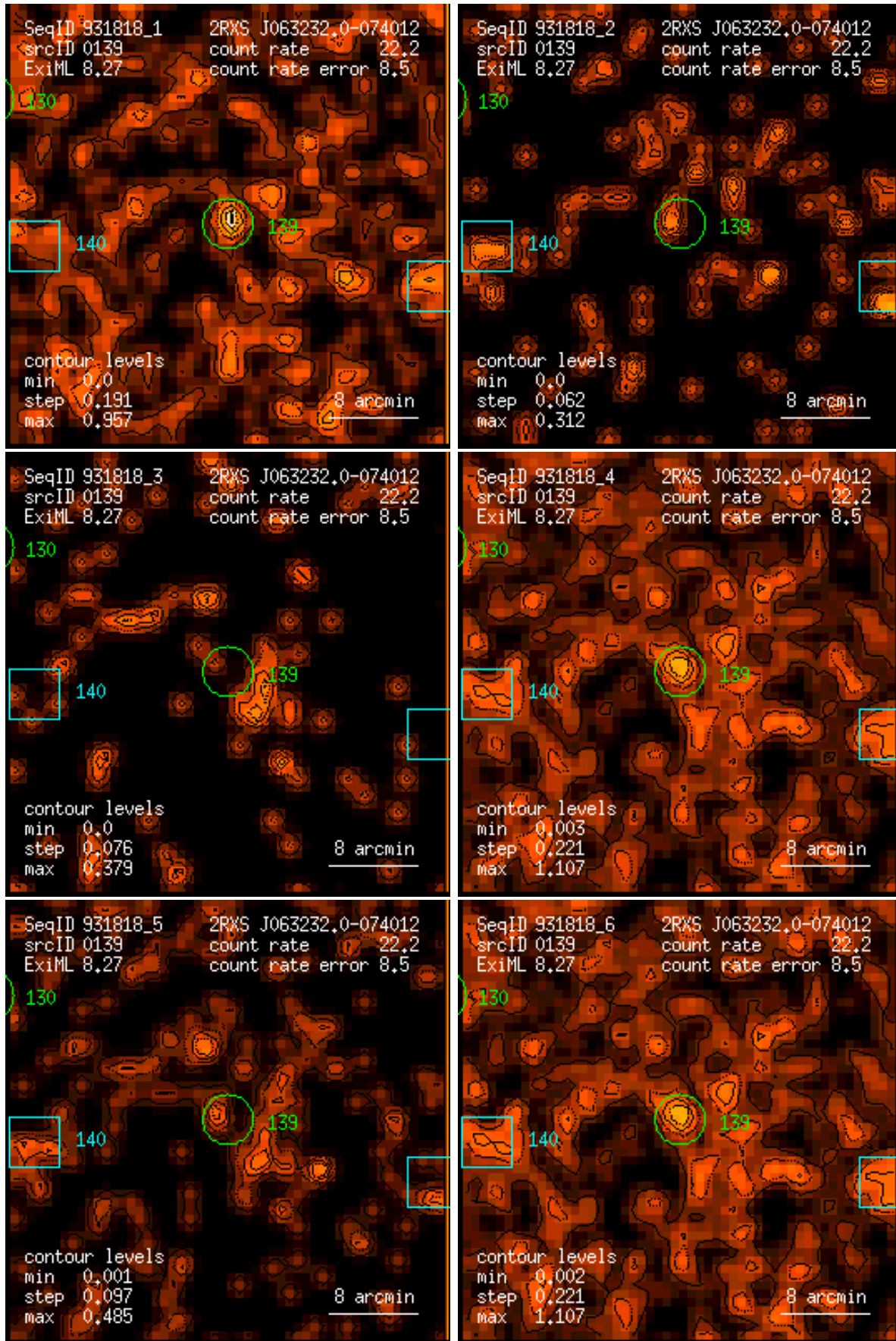
Figure 139: RASS 931818: detection 0139: band rate images, Gaussian filter: (1) PSPC channels 11 – 41, (2) 52 – 90, (3) 91 – 201, (4) 11 – 235, (5) 52 – 201, (6) 11 – 201. Broad band rates in counts/ks. Band rate contour levels in counts/ks/arcmin 2 .
