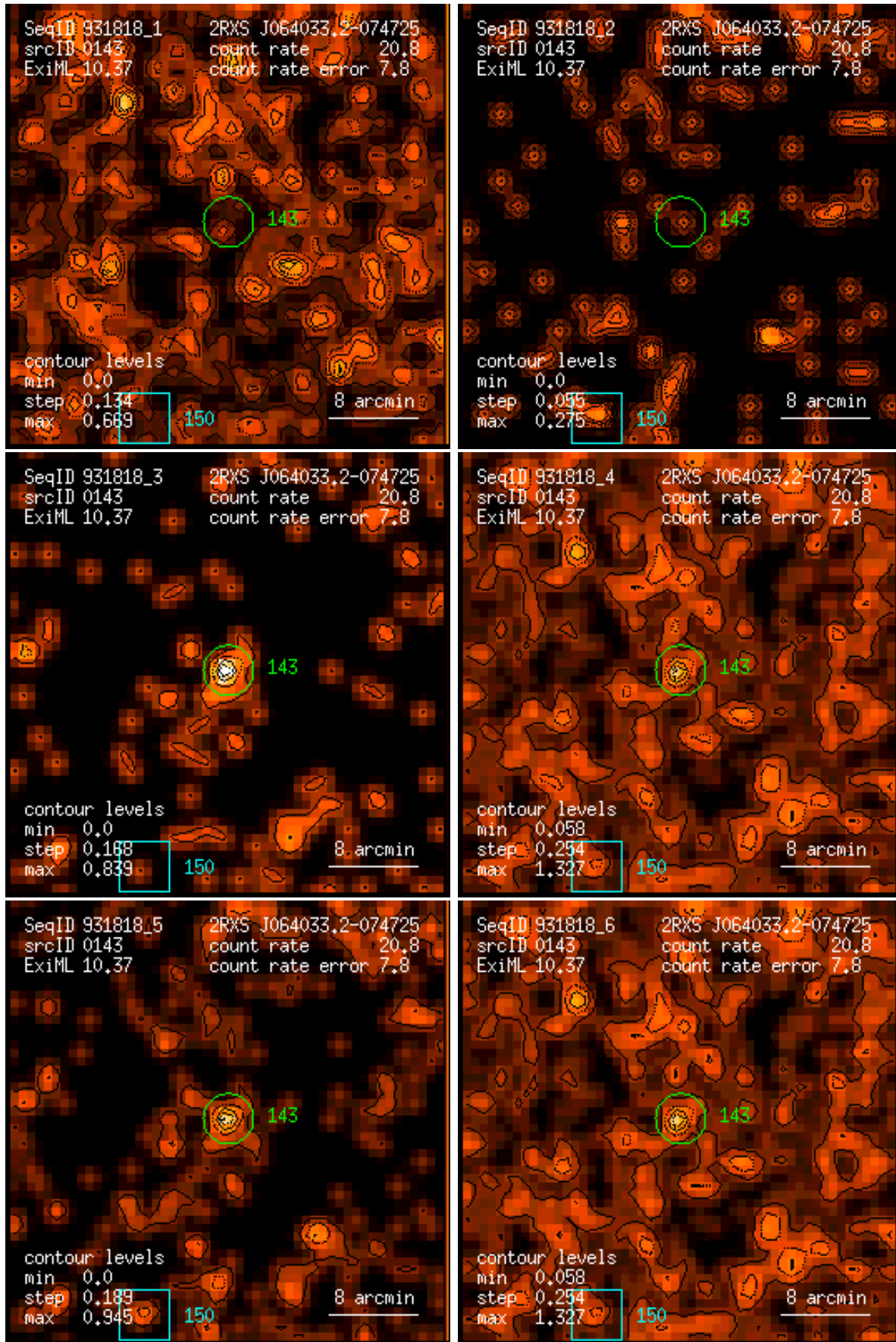
Figure 143: RASS 931818: detection 0143: band rate images, Gaussian filter: (1) PSPC channels 11 – 41, (2) 52 – 90, (3) 91 – 201, (4) 11 – 235, (5) 52 – 201, (6) 11 – 201. Broad band rates in counts/ks. Band rate contour levels in counts/ks/arcmin 2 .
