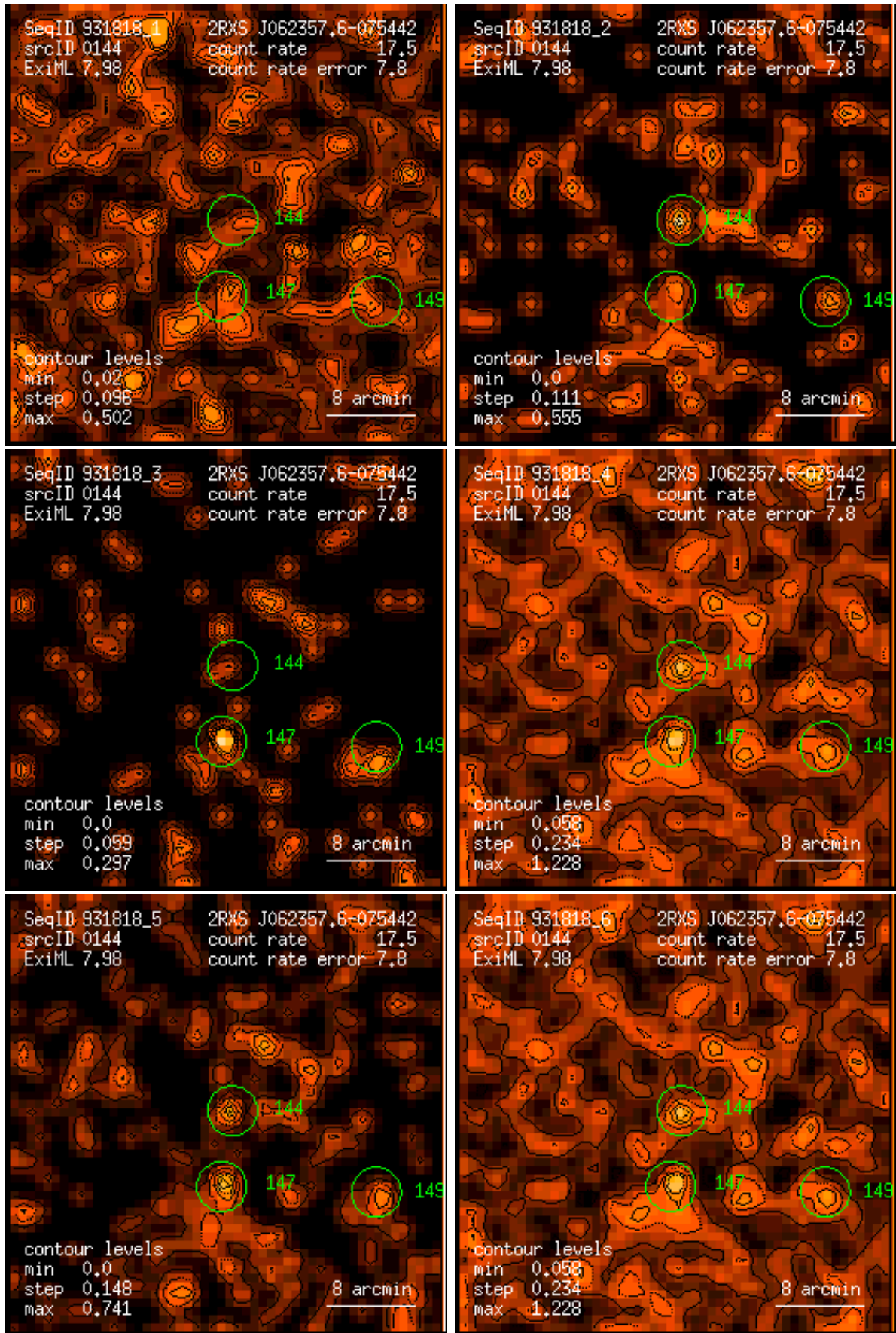
Figure 144: RASS 931818: detection 0144: band rate images, Gaussian filter: (1) PSPC channels 11 – 41, (2) 52 – 90, (3) 91 – 201, (4) 11 – 235, (5) 52 – 201, (6) 11 – 201. Broad band rates in counts/ks. Band rate contour levels in counts/ks/arcmin 2 .
